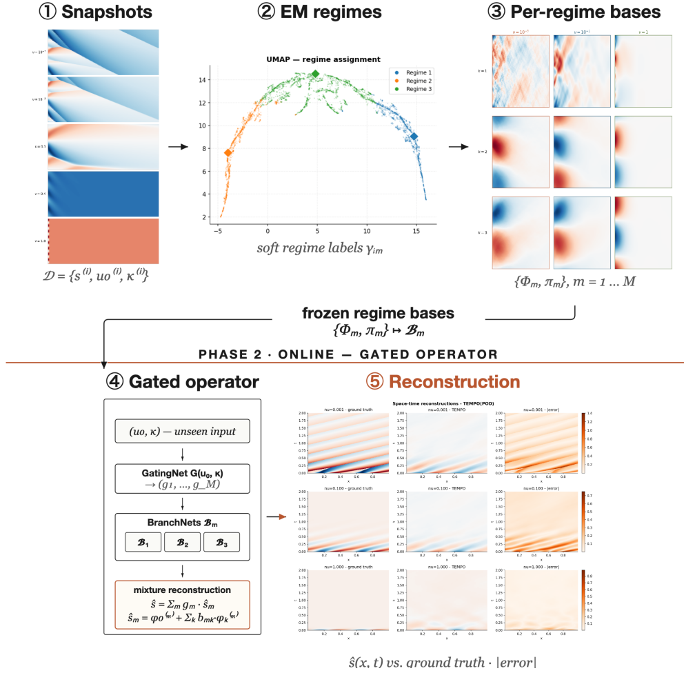
Figure 2: TEMPO pipeline. Phase 1 (offline): snapshots are soft-assigned to M regimes via EM, and a dedicated basis \{\Phi_m\} is fitted per regime. Phase 2 (online): a GatingNet routes each input to regime weights; M BranchNets predict expansion coefficients; the output is a weighted sum of local reconstructions.
