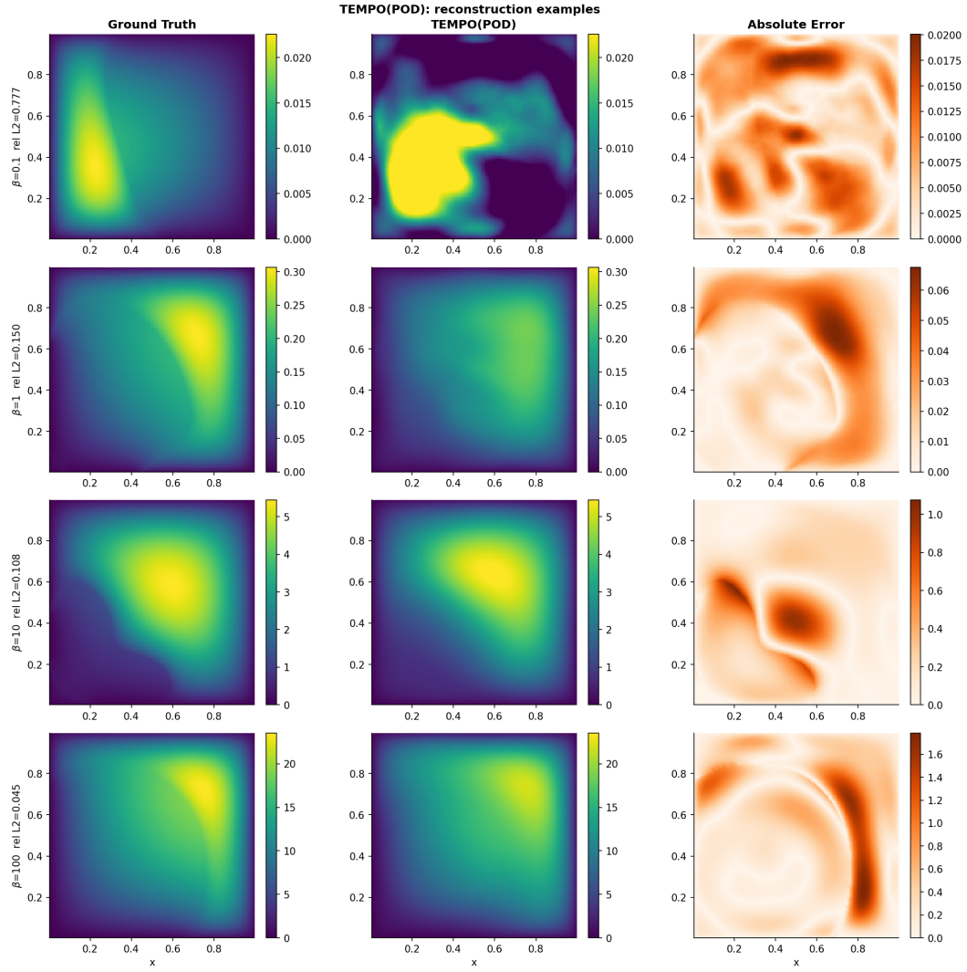
Figure 20: TEMPO(POD) on 2D Darcy flow ( M=5 ): ground truth ( left ), prediction ( center ), point-wise absolute error ( right ).
