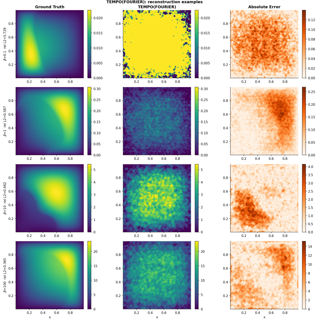
Figure 21: TEMPO(FOURIER) on 2D Darcy flow ( M=5 ). Layout as in Figure 20.
