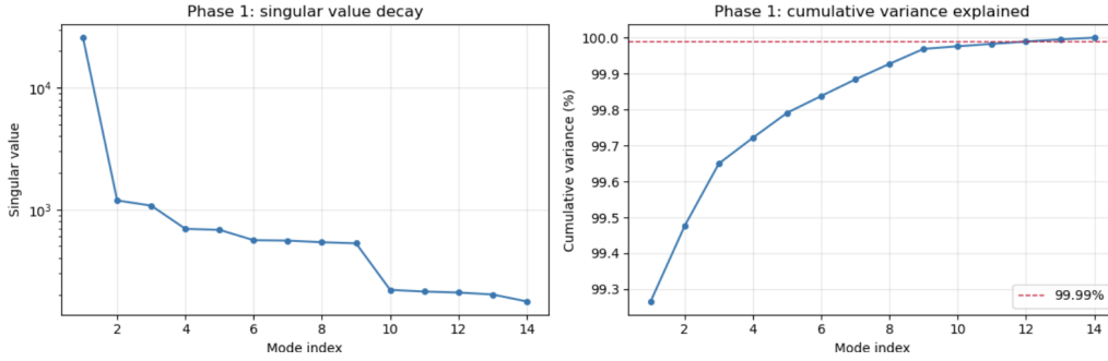
Figure 5: Global POD basis on 1D Burgers' ( \nu=1.0 ): singular value spectrum ( left ) and cumulative explained variance ( right ).
