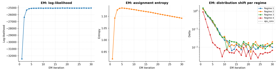
Figure 22: TEMPO(POD) EM convergence on 2D Navier-Stokes ( M=4 ).
