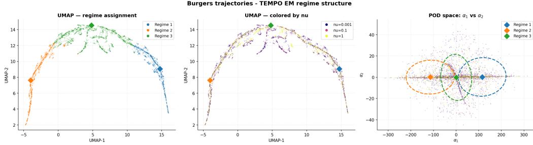
Figure 16: TEMPO(NeuralPOD) on 1D Burgers' ( M=3 , H=0.23 , cf. H=0.84 for POD). Layout as in Figure 4.
