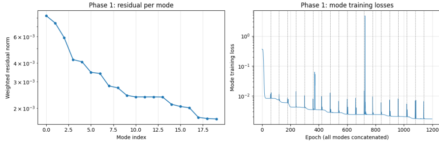
Figure 6: Fourier NeuralPOD basis on 1D Burgers' ( \nu=1.0 ): weighted residual norm versus greedy mode count.
