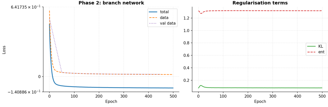
Figure 23: Online training dynamics for TEMPO(POD) on 2D Navier-Stokes ( M=4 ).
