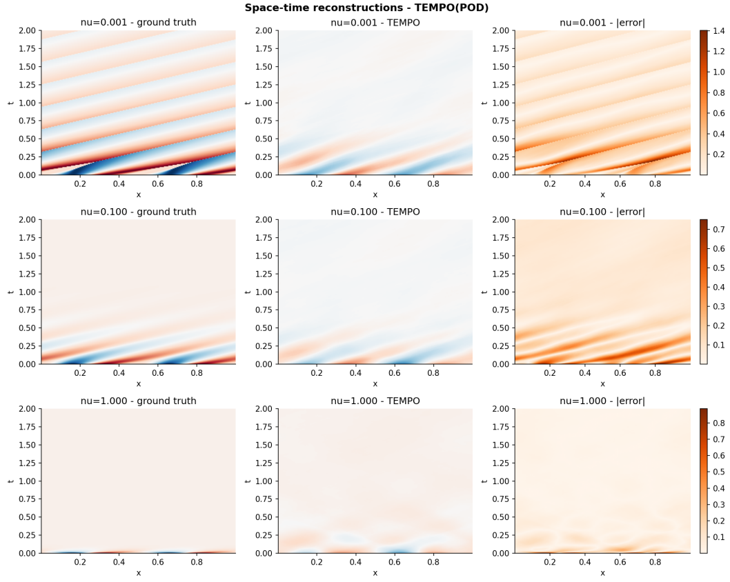
Figure 17: TEMPO(POD) on 1D Burgers' ( M=3 ): ground truth ( left ), prediction ( center ), point-wise absolute error ( right ).
