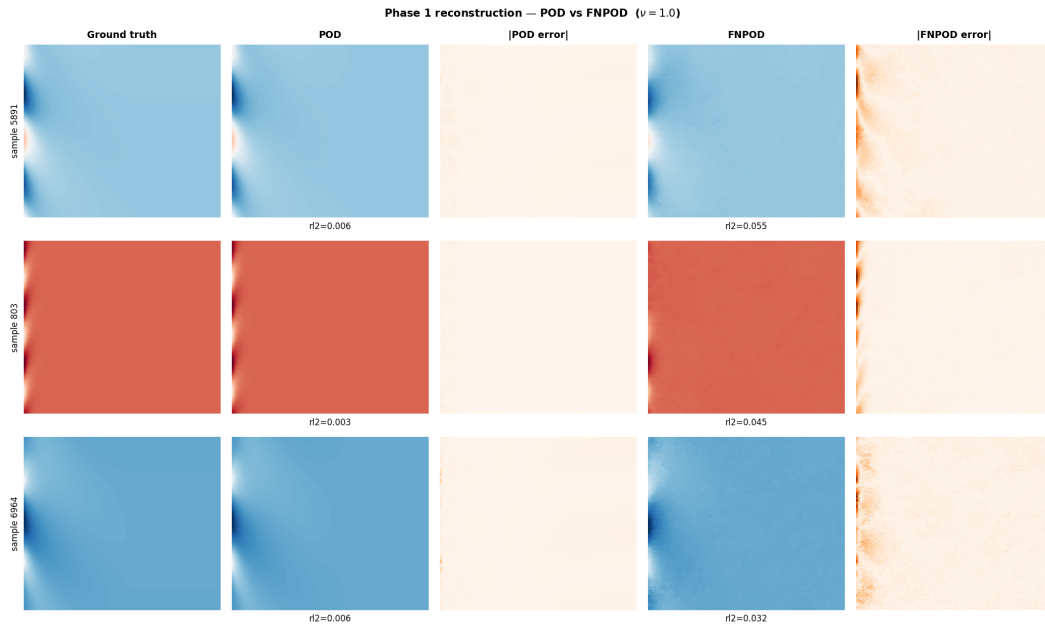
Figure 11: Phase 1 reconstruction comparison on 1D Burgers' ( \nu=1.0 ). Each row shows one sample: ground truth, POD reconstruction, |\text{POD error}| , Fourier NeuralPOD reconstruction, |\text{FNPOD error}| .
