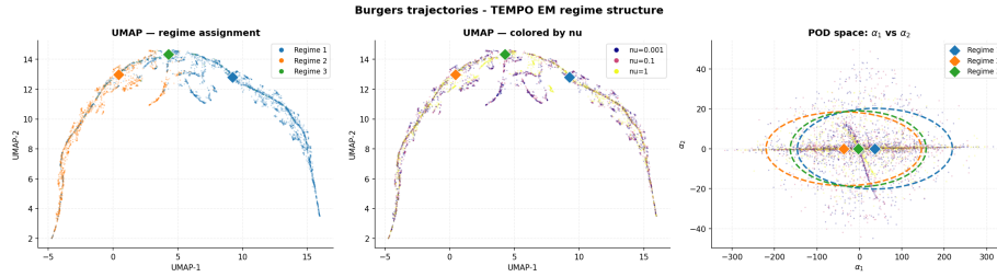
Figure 3: TEMPO(POD) regime structure on 1D Burgers' ( M=3 , 20 EM iterations). Left: UMAP [20] colored by regime. Center: same embedding colored by \nu . Right: GMM fit in POD coefficient space ( \alpha_1, \alpha_2 ); stars mark regime centroids \mu_m .
