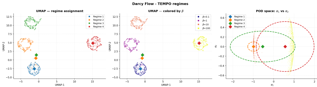
Figure 18: TEMPO(POD) on 2D Darcy flow ( M=4 , H=0.75 , \pi=(0.22, 0.28, 0.28, 0.22) ). Layout as in Figure 3.
