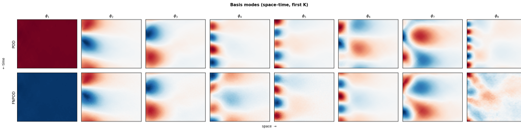
Figure 9: First K basis modes on 1D Burgers' ( \nu=0.01 ): POD ( top ) vs. Fourier NeuralPOD ( bottom ).
