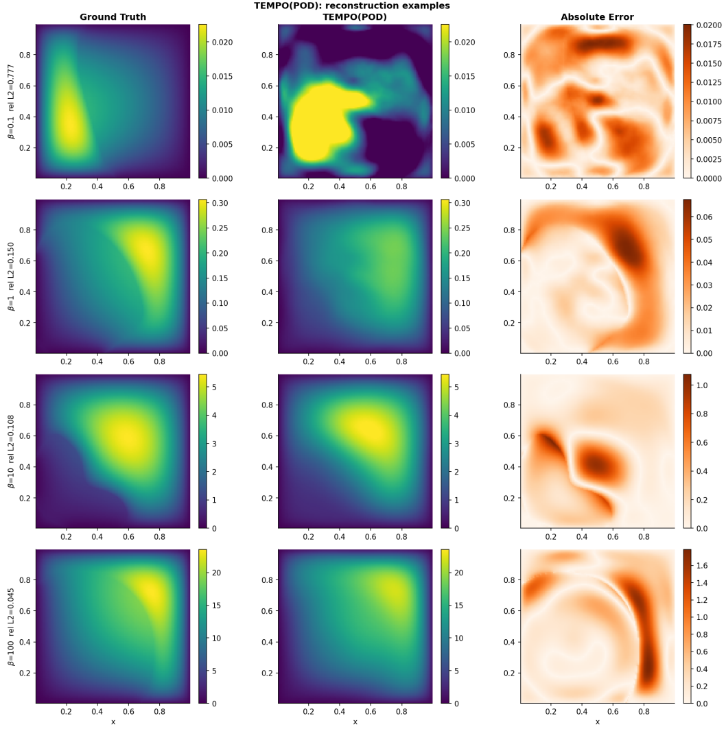
Figure 20: TEMPO(POD) on 2D Darcy flow ( M=5 ): ground truth ( left ), prediction ( centre ), point-wise absolute error ( right ).
