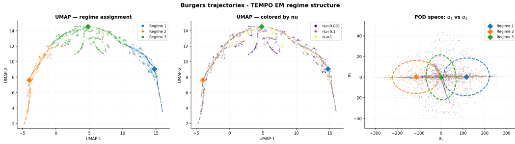
Figure 17: TEMPO(NeuralPOD) on 1D Burgers' ( M=3 , H=0.23 , cf. H=0.84 for POD). Layout as in Figure 3.
