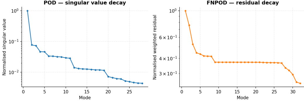
Figure 7: POD singular-value decay ( left ) and Fourier NeuralPOD residual decay ( right ) on 1D Burgers' ( \nu=1.0 ).
