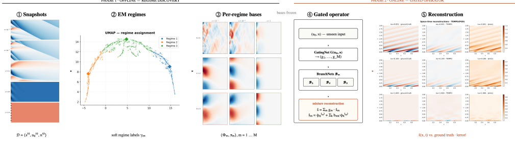
Figure 2: TEMPO pipeline. Phase 1 (offline): snapshots are soft-assigned to M regimes via EM, and a dedicated basis \{\Phi_m\} is fitted per regime. Phase 2 (online): a GatingNet routes each input to regime weights; M BranchNets predict expansion coefficients; the output is a weighted sum of local reconstructions.
