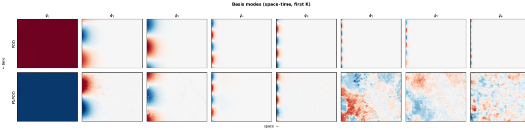
Figure 8: First K basis modes on 1D Burgers' ( \nu=1.0 ): POD ( top ) vs. Fourier NeuralPOD ( bottom ).
