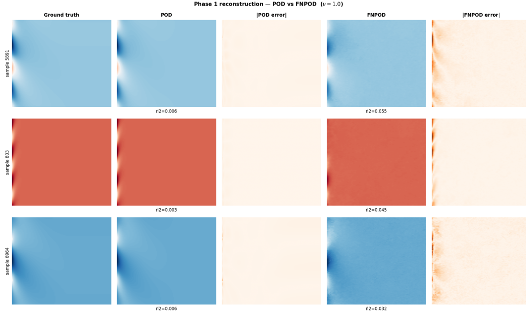
Figure 10: Phase 1 reconstruction comparison on 1D Burgers' ( \nu=1.0 ). Each row shows one sample: ground truth, POD reconstruction, |\text{POD error}| , Fourier NeuralPOD reconstruction, |\text{FNPOD error}| .
