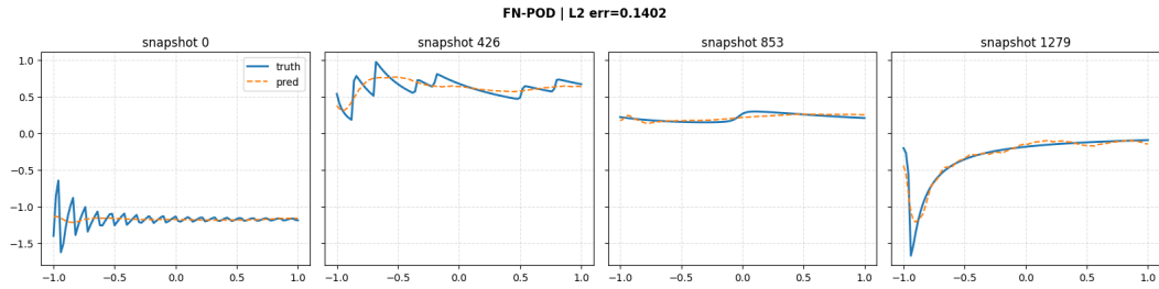
Figure 6: Learned Fourier NeuralPOD basis functions and representative reconstructions on 1D Burgers' ( \nu=1.0 ).
