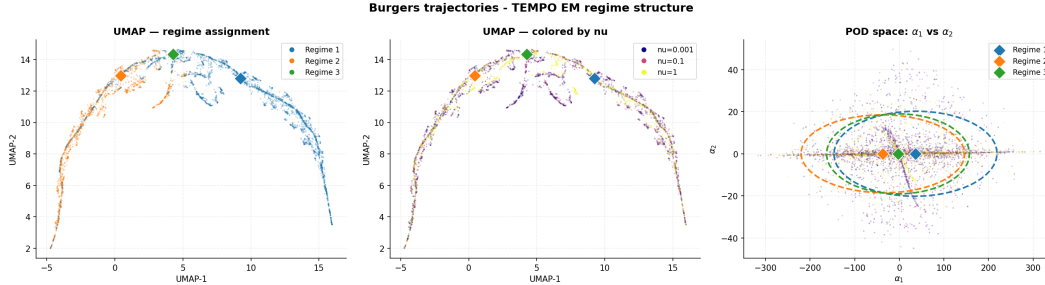
Figure 3: TEMPO(POD) regime structure on 1D Burgers' ( M=3 , 20 EM iterations). Left: UMAP coloured by regime. Centre: same embedding coloured by \nu . Right: GMM fit in POD coefficient space (\alpha_1, \alpha_2) ; stars mark regime centroids \mu_m .
