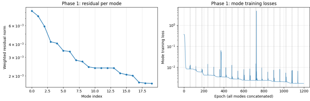
Figure 5: Fourier NeuralPOD basis on 1D Burgers' ( \nu=1.0 ): weighted residual norm versus greedy mode count.
