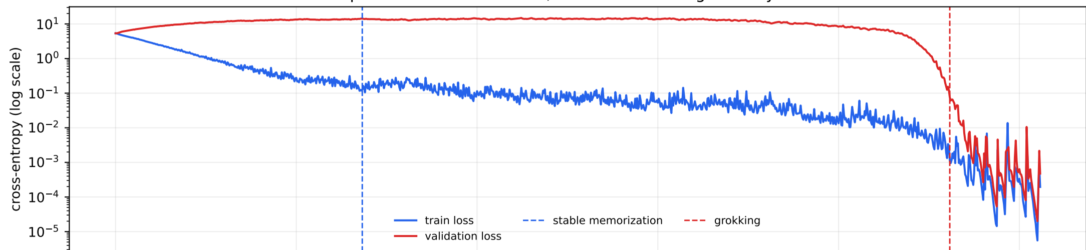
p=211 modular addition, fixed AdamW weight decay 0.5
