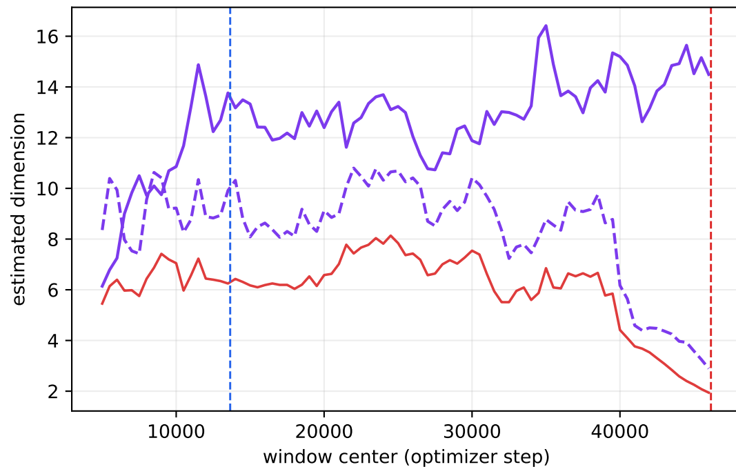
LB arithmetic
