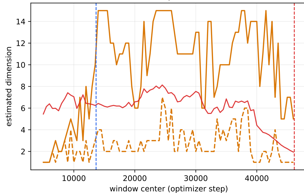
Simplex
