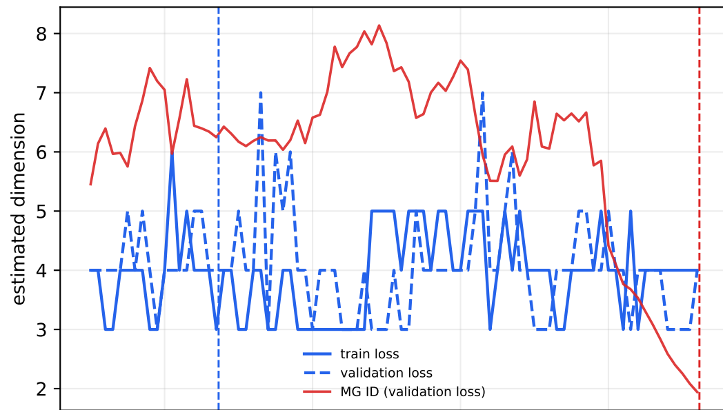
FNN
