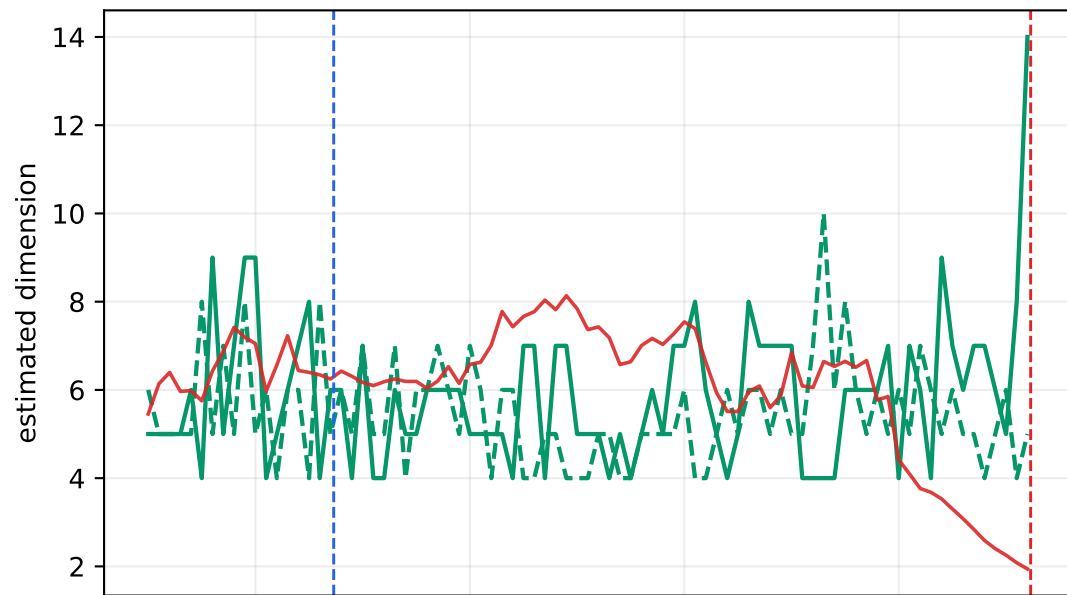
Cao
