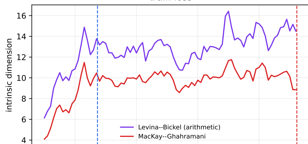
Core scalar observers: Levina--Bickel and MacKay--Ghahramani (linear trend removed independently in each window)
