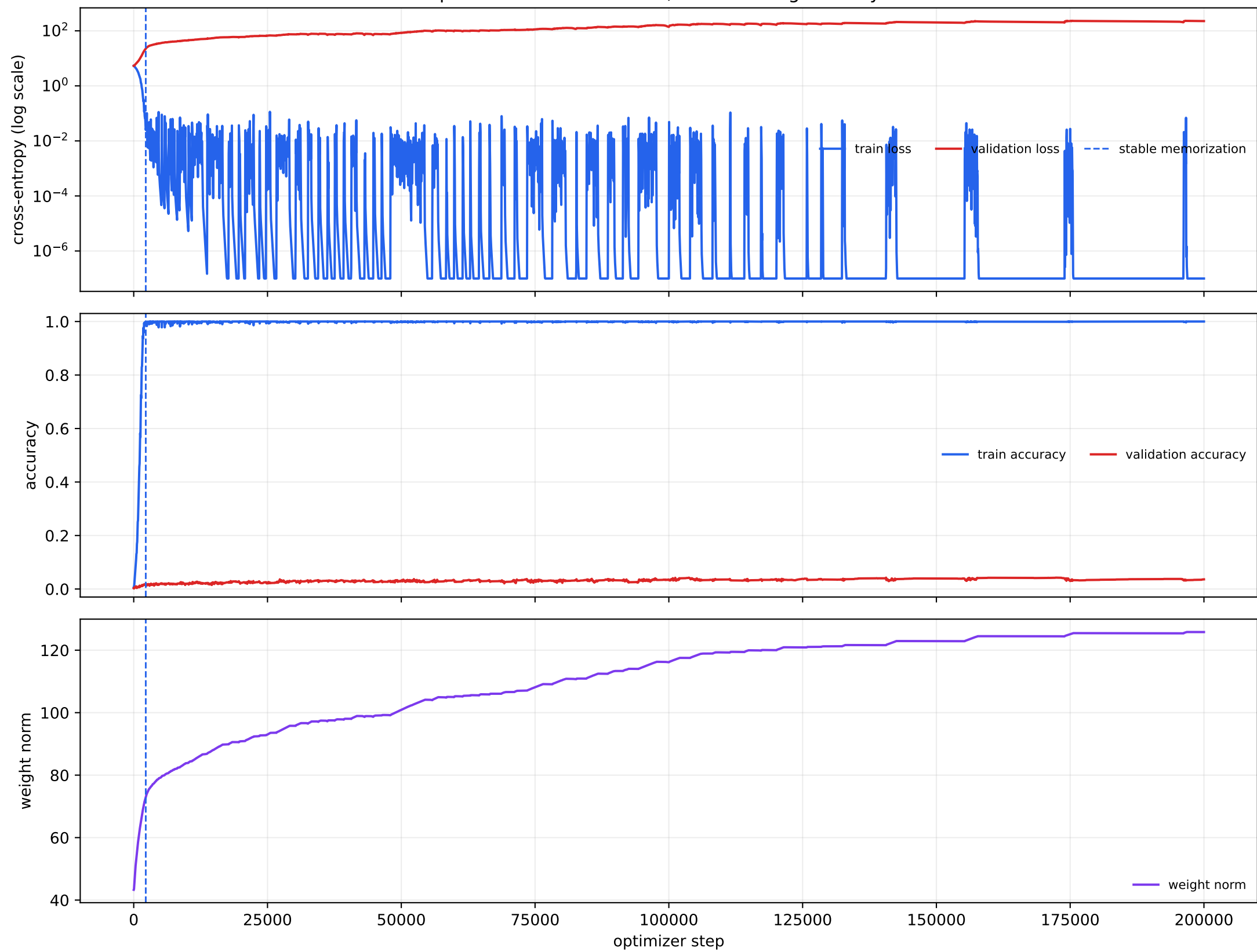
p=211 modular addition, AdamW weight decay 0
