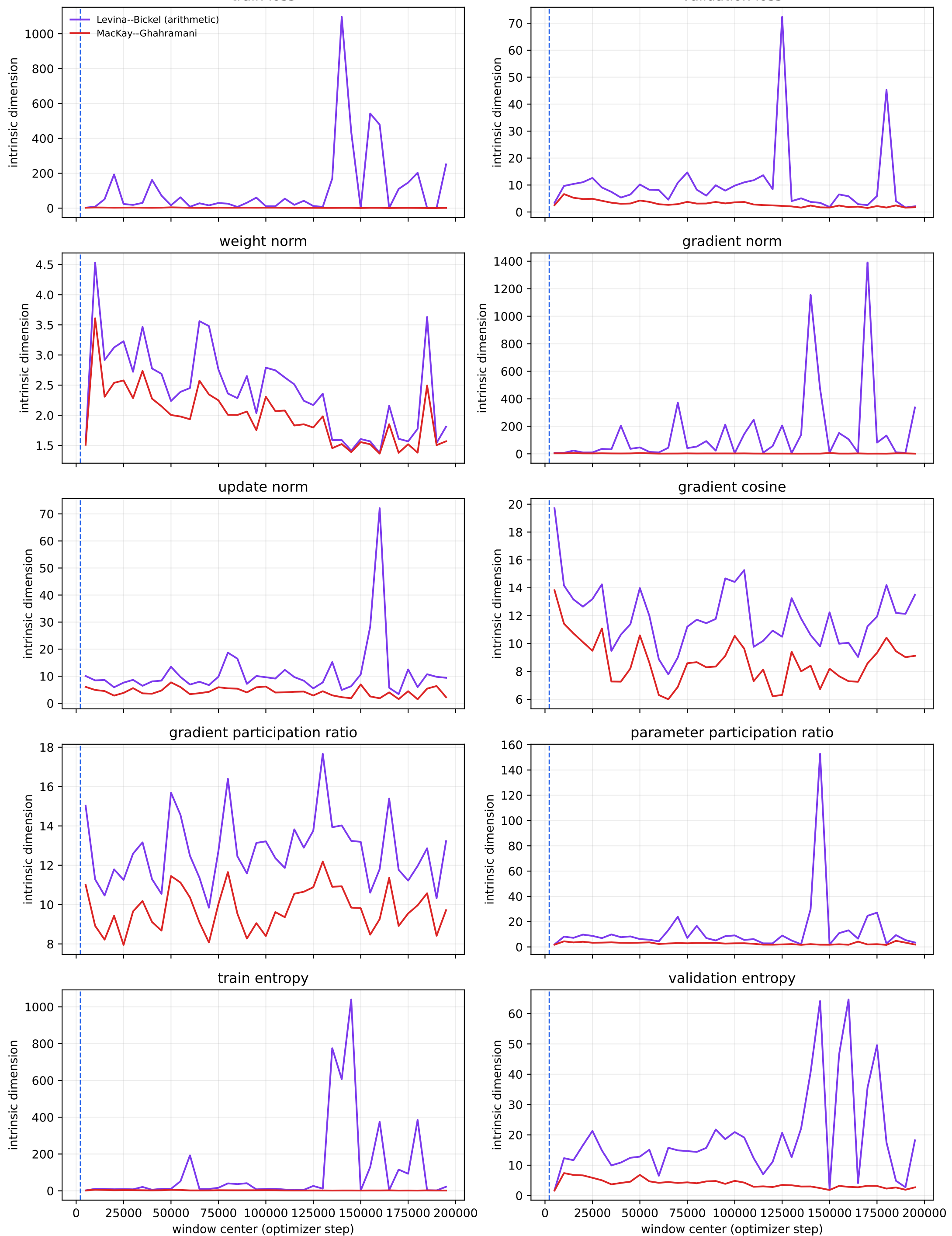
Core scalar observers: Levina--Bickel and MacKay--Ghahramani (linear trend removed independently in each window)
