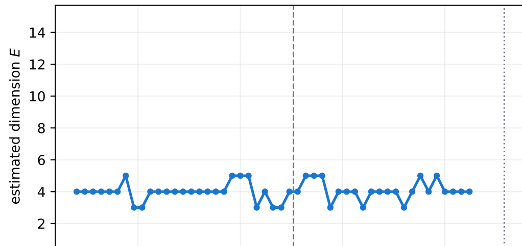
FNN
