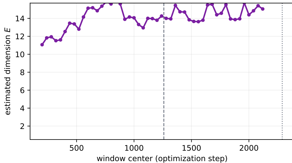
dashed: start of LR cooldown; dotted: extension start
