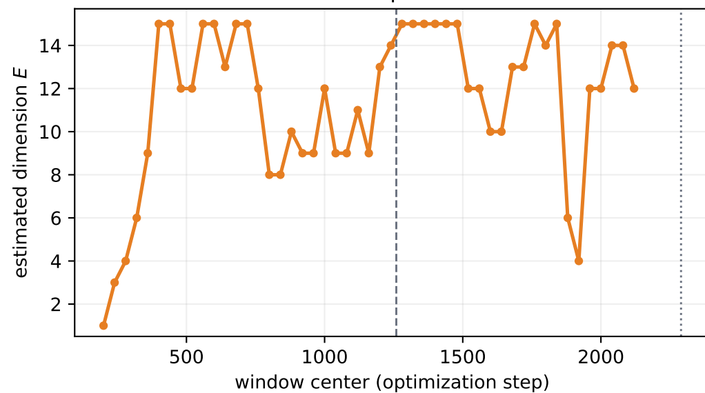
Simplex
