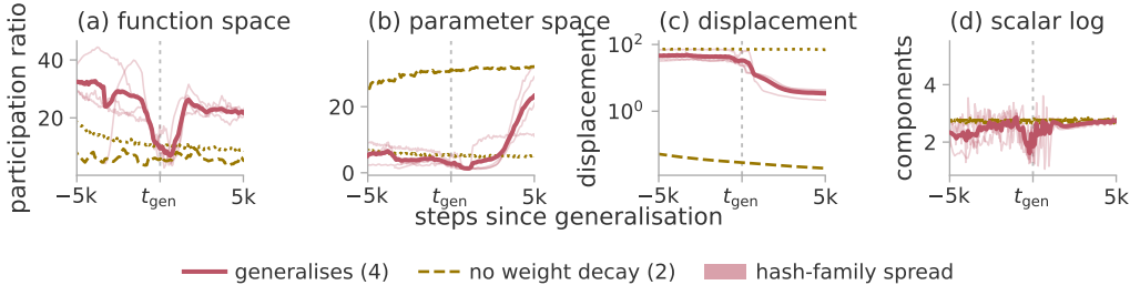
Figure 2: Simplification of the trajectory at generalisation, measured against two controls. Three regularised seeds of modular addition and one S_5 composition, against the same two configurations without weight decay, which memorise and stay at chance accuracy. Colour is the regime of table 1; the thick line is the mean of the four runs that generalise, and each control is aligned on the generalisation step of its matched run. The statistic in (a)–(c) is \text{PR}^{\text{det}} , an effective rank: none of these runs recurs, so none supports reading a dimension. Windows are 600 optimiser steps, 300 for S_5 , plotted at their midpoint; the band on (a) and (b) is the two-hash disagreement (Appendix I). Panel (d) is a different measurement on the same midpoints: the delay estimate of section 7.3 on the parameter-norm log.
