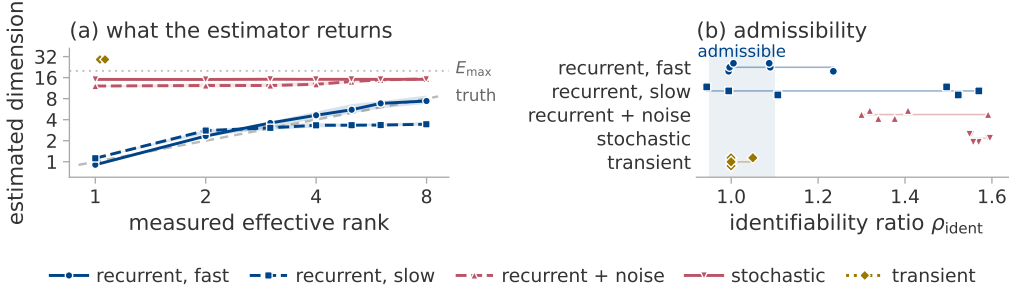
Figure 1: Recovery of the active dimension in each regime, and separation of the regimes without ground truth. The evaluation of section 5.4: a frozen tanh network on the digits data, a linear head confined to ten directions of which r are excited, five of the nine excitation cases; colour is the regime of table 1. (a) The estimate against the measured effective rank, which the construction holds at r ; the marker is the median of forty values, four seeds by ten observers, and the band their interquartile range. The dashed diagonal is the truth and the dotted line E_{\max} , a reference and not a bound: no clamping is applied, and the transient case lies above it, its seven points piled at x \approx 1.05 because its measured rank is about one at every r . (b) The identifiability ratio on a smaller grid — seed 0, three observers, r \in \{2, 6\} . The transient is the one regime it passes, which is why section 3.4 adds the trend-crossing count.
