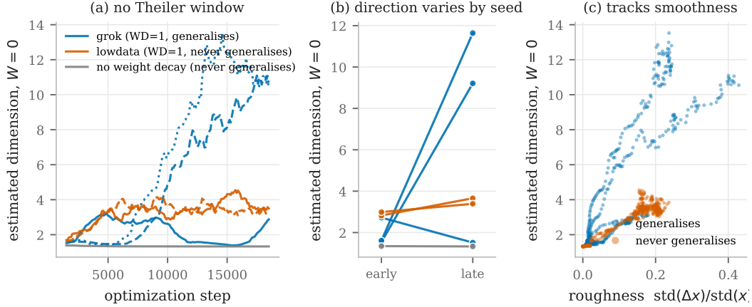
Figure 3: The dimension signal evaluated with no Theiler exclusion. (a) Sliding-window estimates. Line style distinguishes seeds within a family. (b) Median estimate over the first and last third of training. Two of the three generalising runs rise, one falls, and the never-generalising runs at identical weight decay lie between them; the no-weight-decay run is flat at the tangent constant, its apparent monotone decline spanning only 1.34 to 1.33. (c) The estimate against a roughness ratio that involves no embedding.
