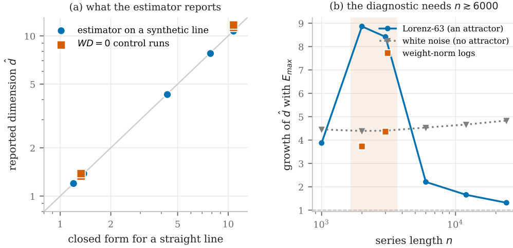
Figure 2: (a) Dimension reported by the estimator against the closed form of Proposition 1, on logarithmic axes with the identity line shown. A synthetic straight line and the WD = 0 control runs both lie on the prediction. (b) Growth of the estimate between E_{max} = 5 and E_{max} = 30 , against series length. A quantity that is a property of the data does not depend on the space it is measured in, so a value near unity is the signature of a resolvable attractor. The Lorenz reference reaches it only beyond n \approx 6000 ; inside the shaded band, which is the length training logs provide, it scores worse than both white noise and the logs, so the diagnostic cannot discriminate there.
