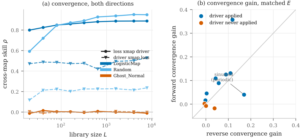
Figure 8: Forward against reverse cross mapping, both directions at a matched embedding dimension. (a) Skill against library size. The forward map converges for the coupled runs while the reverse remains flat, and both directions are flat for the ghost. (b) Convergence gain in the two directions. Coupled runs lie above the diagonal, ghost runs sit at the origin, and the exception is the smooth periodic driver of section 5.3.
