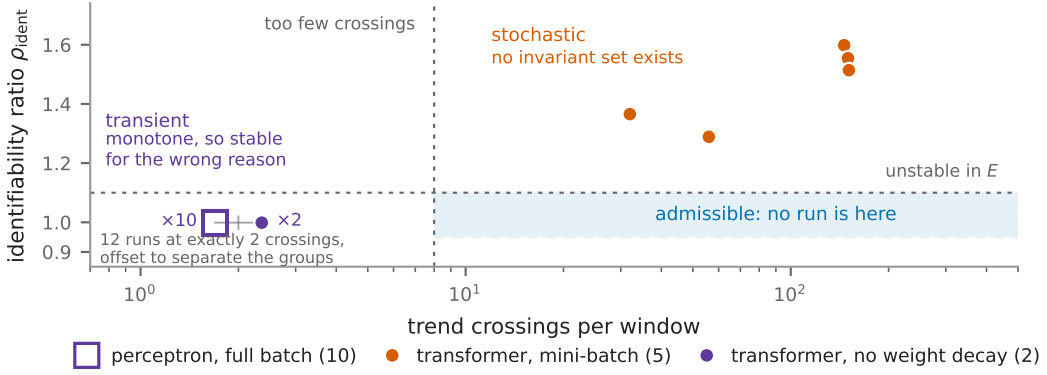
Figure 3: Every training log of section 7 in the plane of the two diagnostics, one point per run: seven transformer runs of 120 000 steps observed through the parameter norm, and ten perceptron runs of 100 000 steps observed through the training loss. The vertical axis is the identifiability ratio, near unity when the estimate does not depend on the embedding dimension; the horizontal axis is the trend-crossing count, which tests non-monotonicity of the series and not recurrence in the reconstructed space. Twelve of the seventeen runs coincide: all ten perceptron runs and both zero-weight-decay transformer runs have exactly two crossings, with \rho_{\text{ident}} between 0.9975 and 0.9992. Those two groups are drawn with a small offset either side of their true abscissa, which the grey tick marks, and labelled with their multiplicity. The shaded rectangle is where every accurate case of section 6 fell: \rho_{\text{ident}} \leq 1.10 and more than eight crossings. It describes the calibration and is not a validated decision rule; no run of either setting is inside it, and the two settings fail in different corners without reference to any label.
