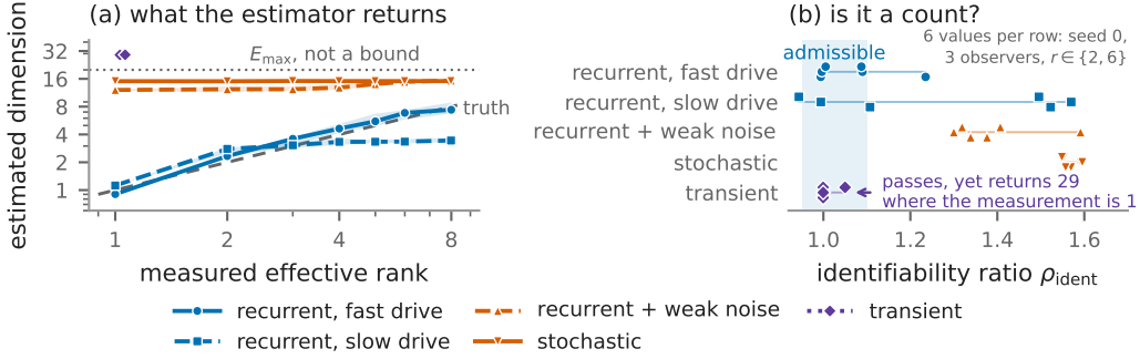
Figure 1: The evaluation of section 5.4: a frozen tanh network on the digits data, a linear head confined to ten directions of which r are excited, five of the nine arms. (a) The estimate against the measured effective rank, which the construction holds at r ; the marker is the median of the forty values behind each point, four seeds by ten observers, and the band their interquartile range. It tracks the truth only under a fast recurrent drive. The seven transient points pile up at x \approx 1.05 because that arm’s measured rank is about one at every nominal r ; that is the measurement, not missing data. (b) The identifiability ratio, which separates the regimes with no ground truth. It is not computed on the runs of (a): the sweep populates it for seed 0, three observers and r \in \{2, 6\} only, so each regime rests on the six values plotted, one sub-row per observer. The transient is the one regime it passes, hence the trend-crossing count of section 3.4.
