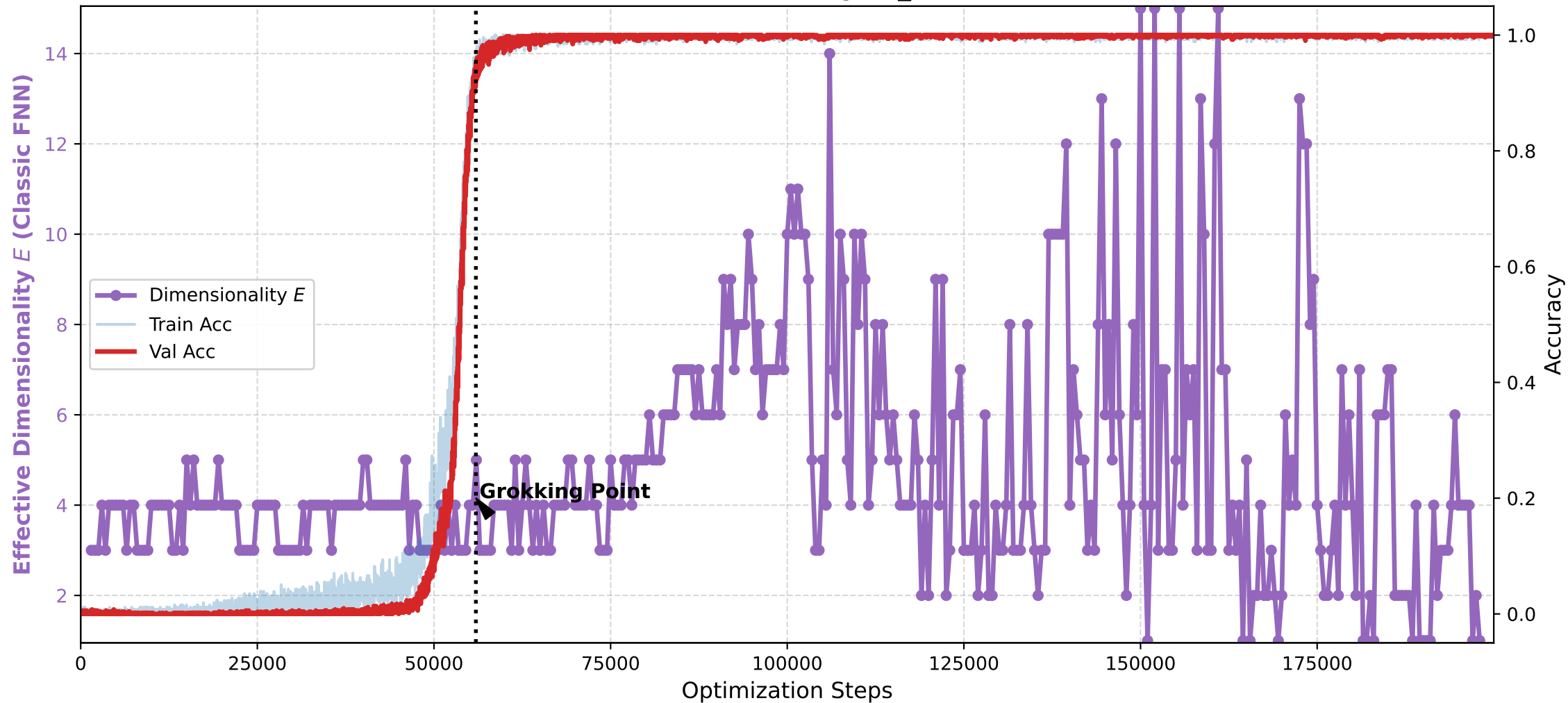
Collapse of Dimensionality during Grokking Method: Classic FNN (Metric: grad_cosine, W=300)
