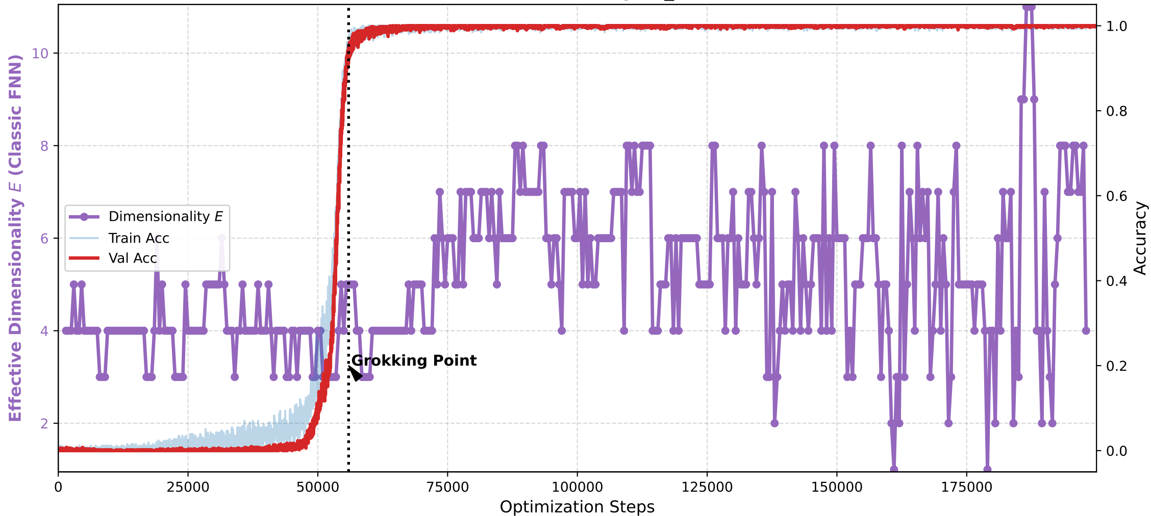
Collapse of Dimensionality during Grokking Method: Classic FNN (Metric: grad_norm, W=300)
