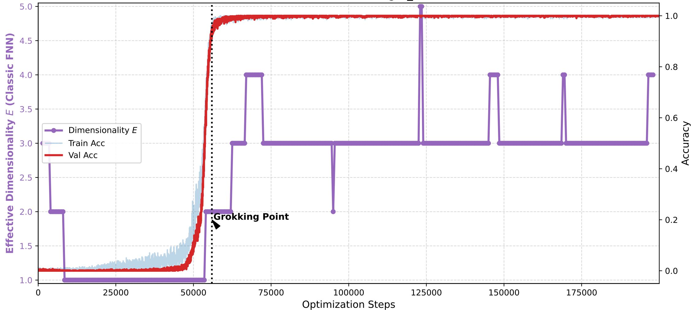
Collapse of Dimensionality during Grokking Method: Classic FNN (Metric: weight_norm, W=300)
