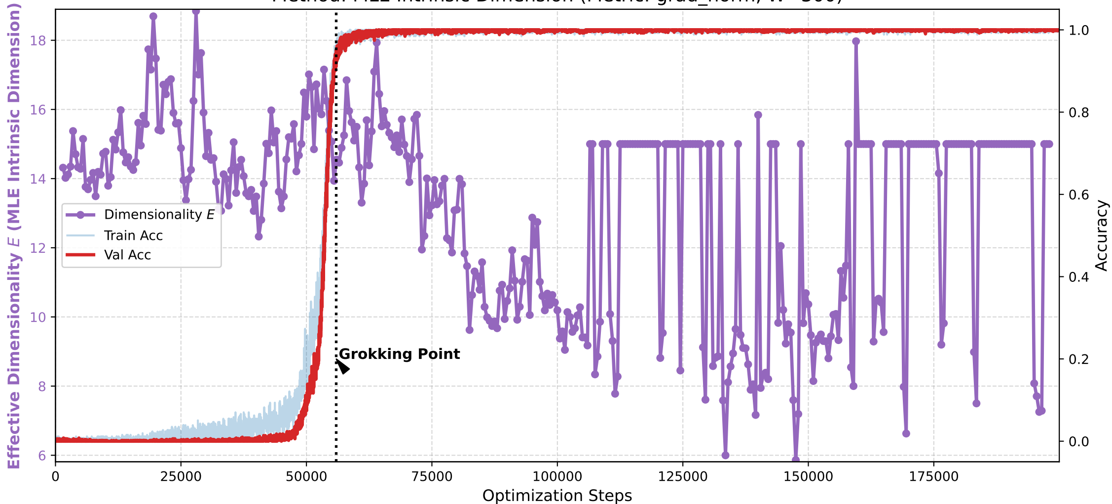
Collapse of Dimensionality during Grokking Method: MLE Intrinsic Dimension (Metric: grad_norm, W=300)
