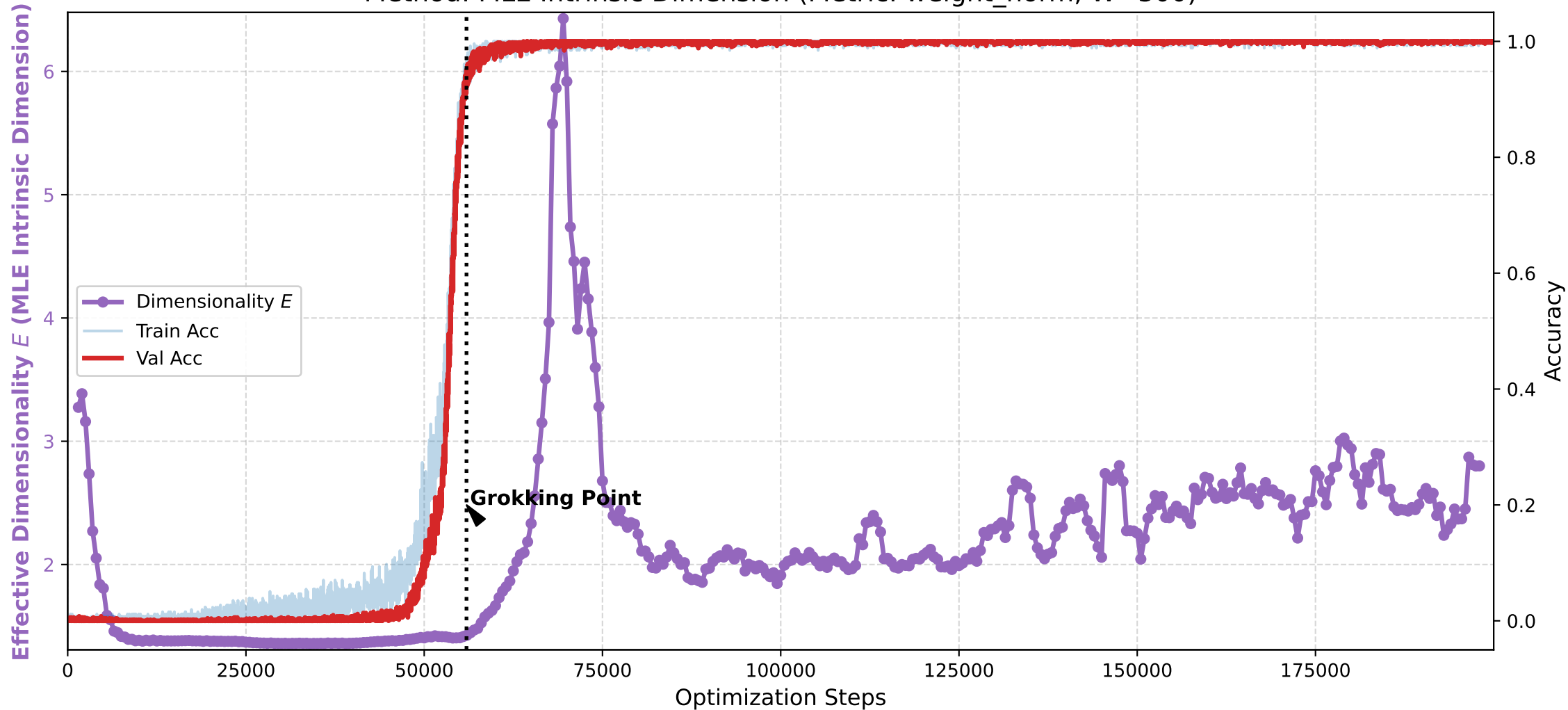
Collapse of Dimensionality during Grokking Method: MLE Intrinsic Dimension (Metric: weight_norm, W=300)
