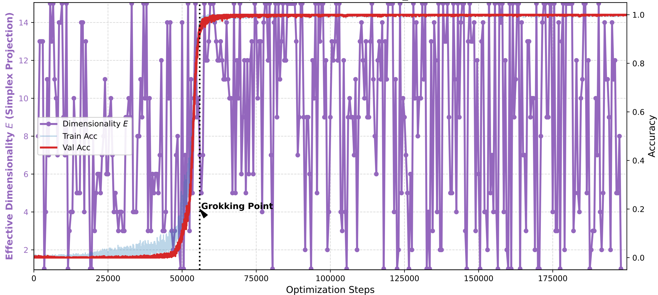
Collapse of Dimensionality during Grokking Method: Simplex Projection (Metric: train_loss, W=300)
