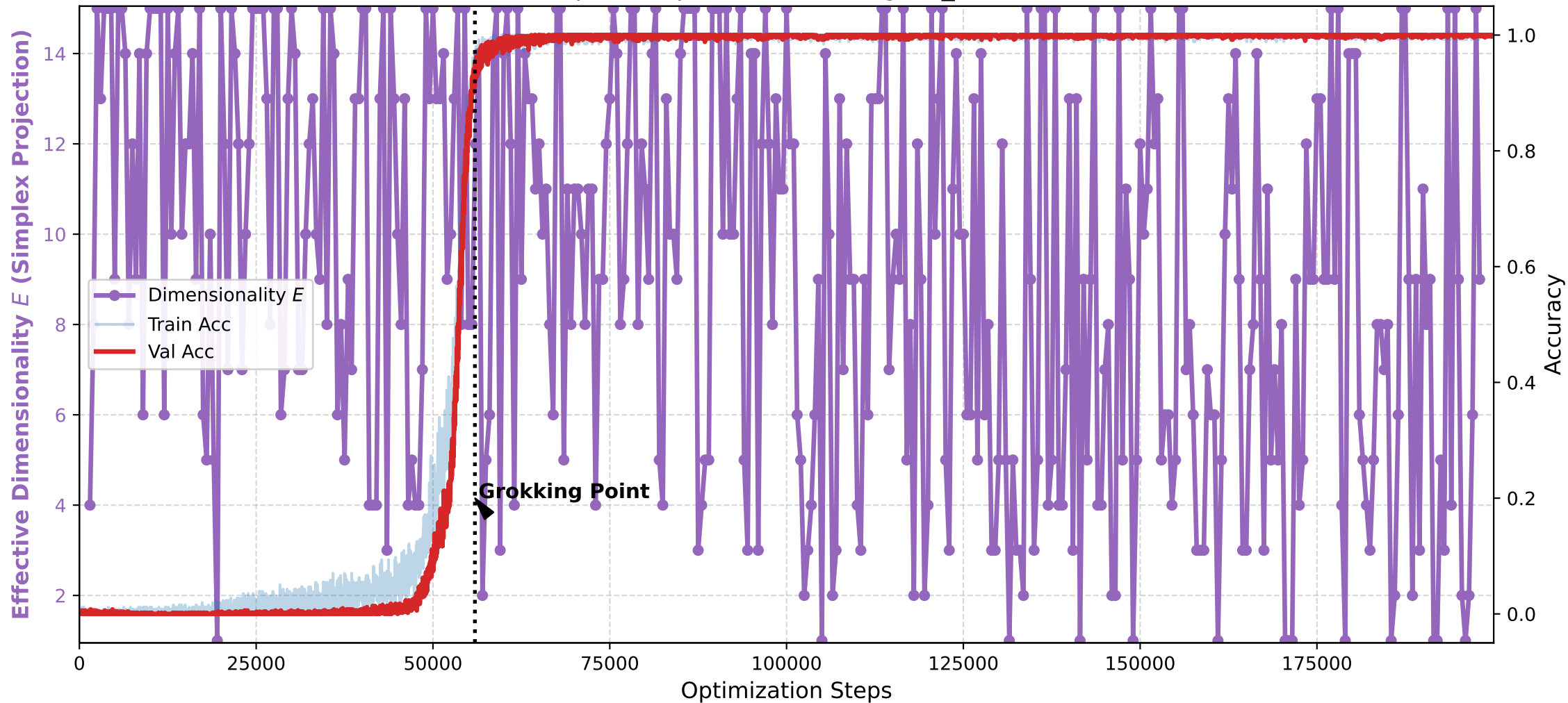
Collapse of Dimensionality during Grokking Method: Simplex Projection (Metric: grad_cosine, W=300)
