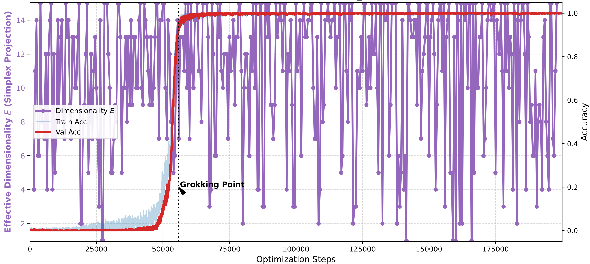
Collapse of Dimensionality during Grokking Method: Simplex Projection (Metric: grad_norm, W=300 )
