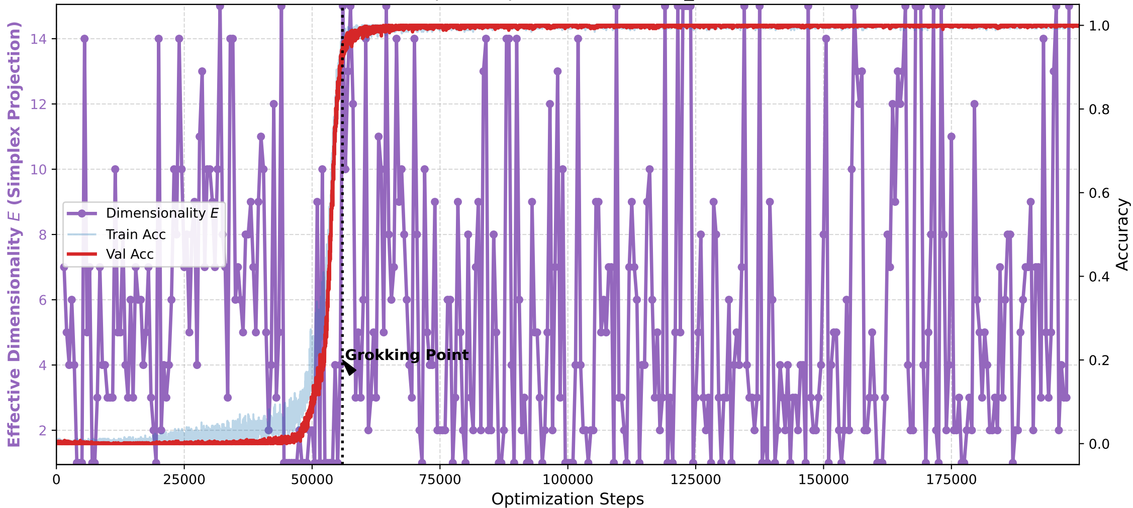
Collapse of Dimensionality during Grokking Method: Simplex Projection (Metric: val_loss, W=300)
