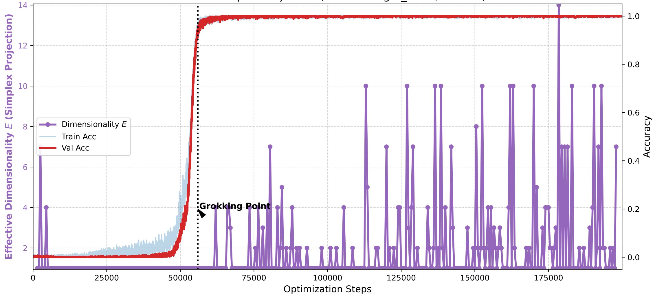
Collapse of Dimensionality during Grokking Method: Simplex Projection (Metric: weight_norm, W=300)
