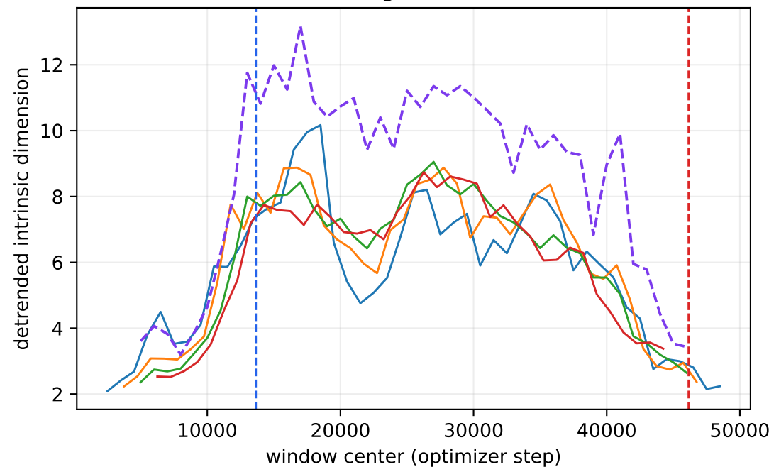
weight norm
