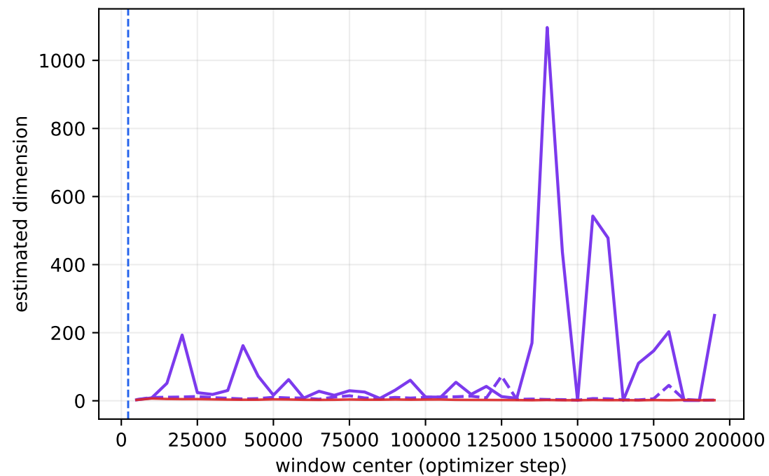
LB arithmetic
