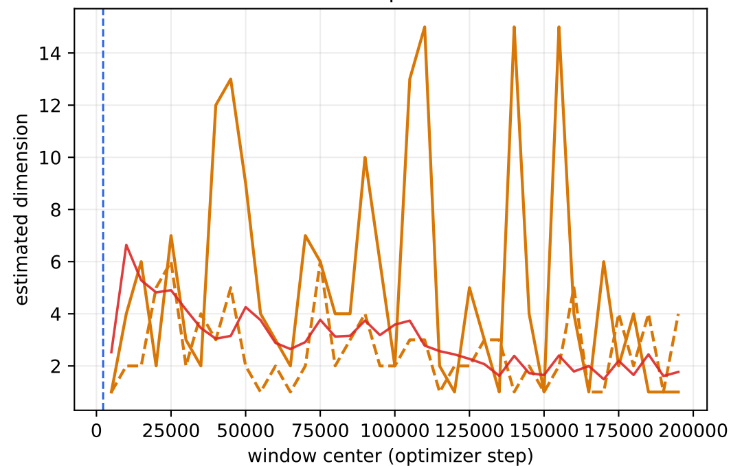
Simplex
