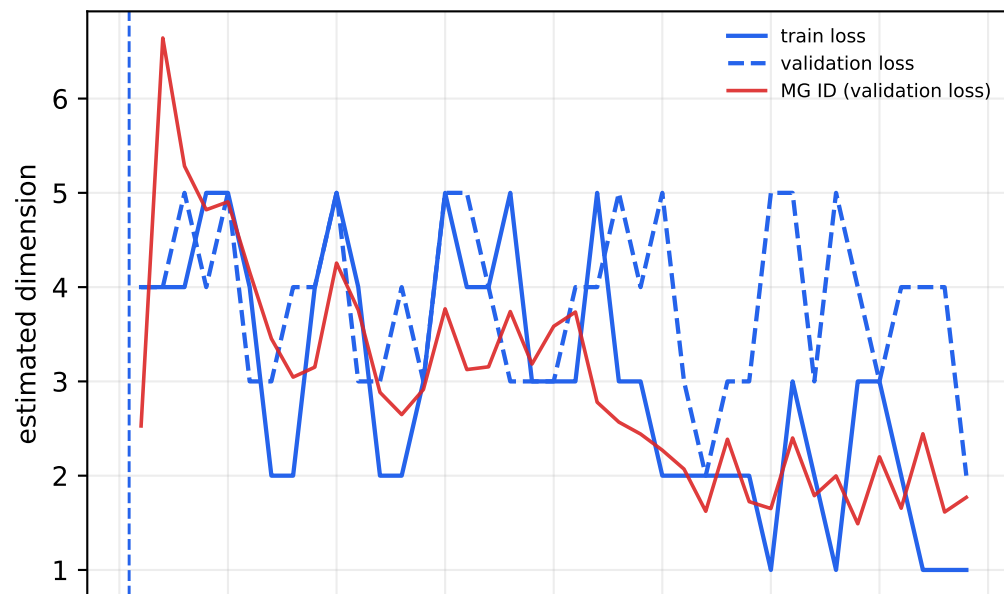
FNN
