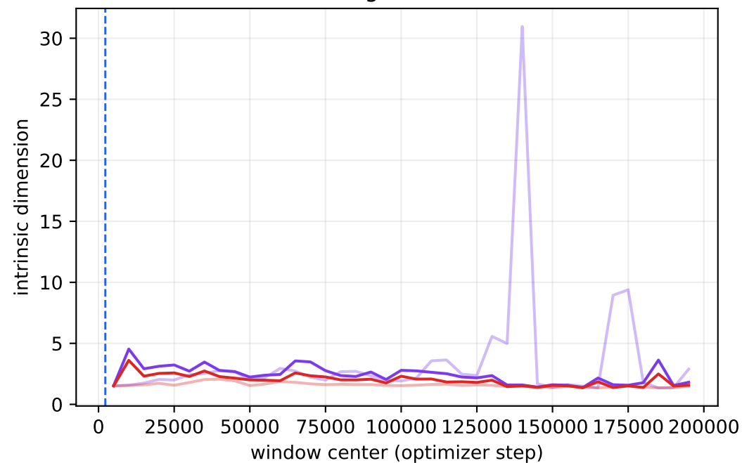
weight norm
