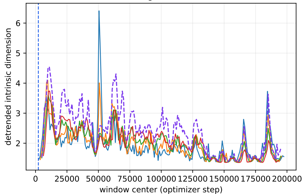
weight norm
