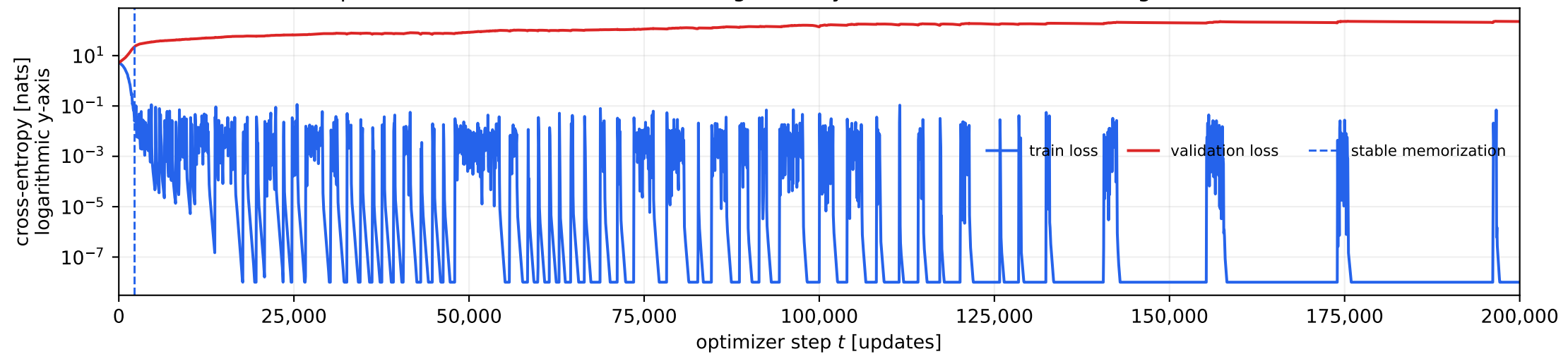
p=211 modular addition, fixed weight decay 0: memorization without generalization
