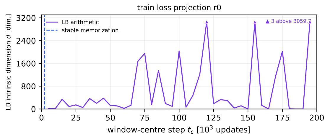
Fixed random projections: LB and MG: Levina-Bickel arithmetic estimate; triangles mark values above the displayed range
