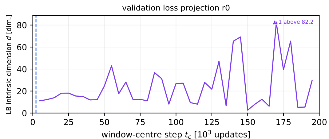
Fixed random projections: LB and MG: Levina-Bickel arithmetic estimate; triangles mark values above the displayed range
