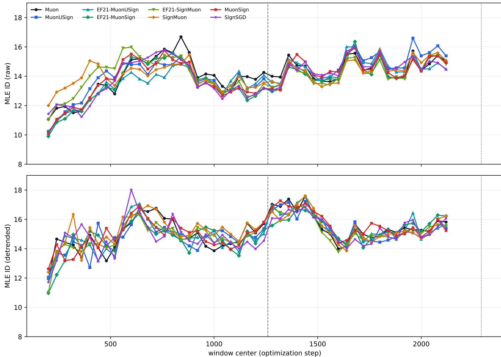
Levina-Bickel MLE trajectories, fixed \tau = 1
