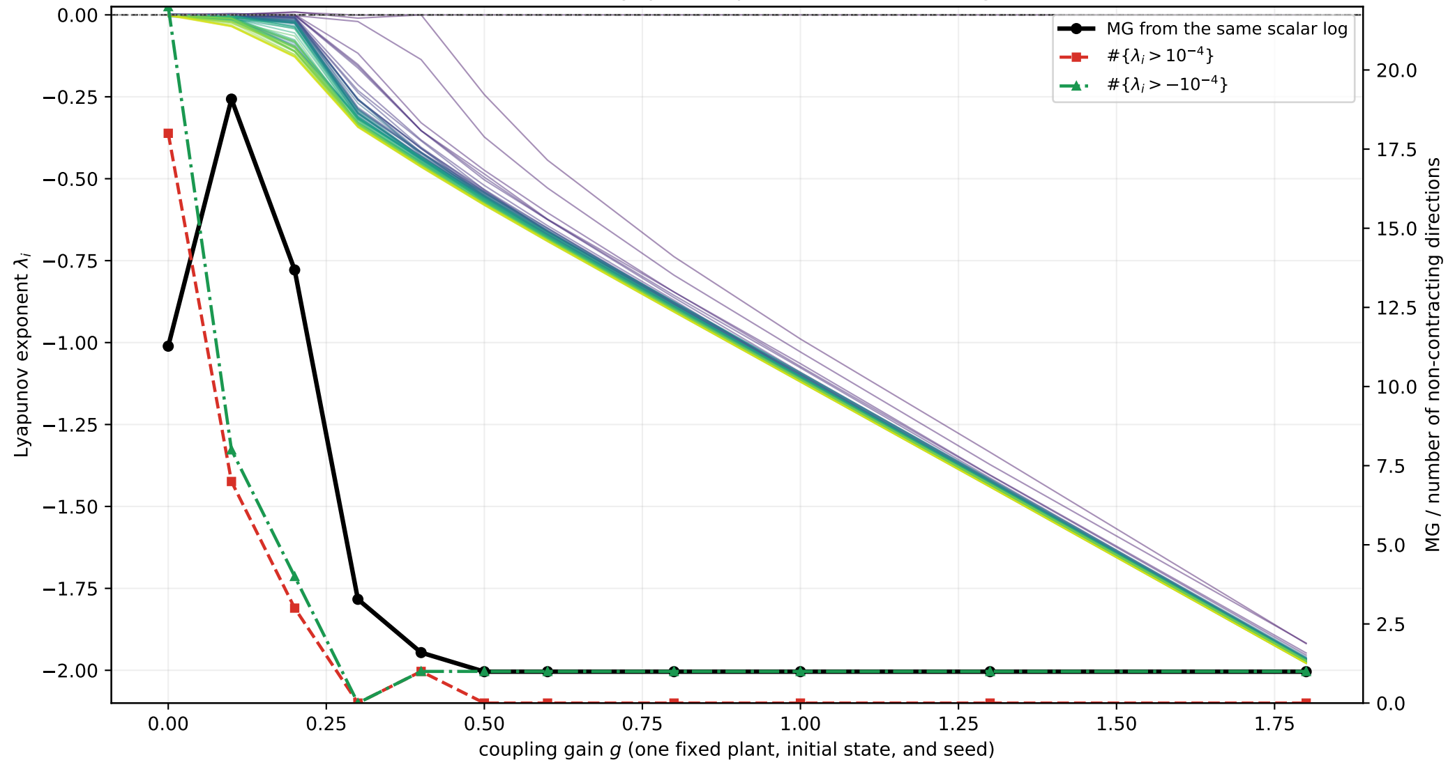
Same-seed full Lyapunov spectrum and scalar-log MG
