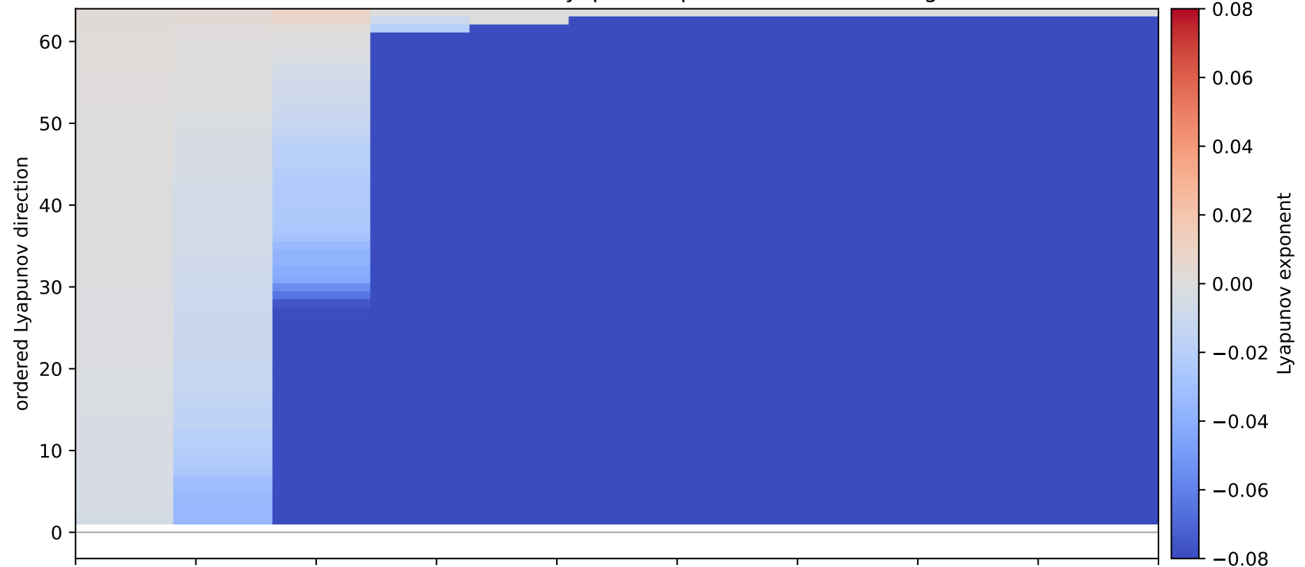
Same seed: full finite-time Lyapunov spectrum and scalar-log MG
