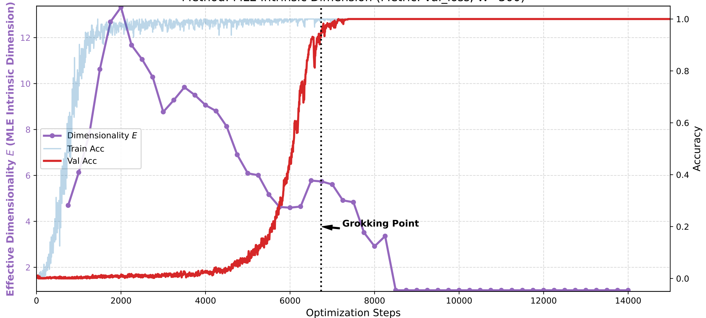
Collapse of Dimensionality during Grokking Method: MLE Intrinsic Dimension (Metric: val_loss, W=300)
