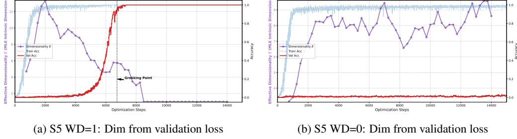
Figure 3: Analysis of the S_5 group. The dimensionality E reconstructed from the validation loss successfully estimates the true algebraic complexity of the algorithm (plateauing at \hat{d} \approx 4 ).
