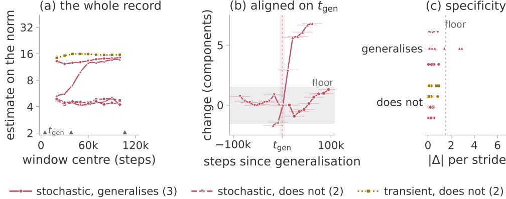
Figure 9: What a frozen-window estimate can and cannot localise. The windowed estimate on the parameter norm for the seven extended runs, under the frozen configuration of section 7.1: nine windows per run of 39 990 optimiser steps, advanced by 10 000, plotted at their centres. Colour is the regime of section 3.3. (a) All sixty-three windows, with the three generalisation steps marked on the axis. (b) The three generalising runs aligned on their own generalisation step, each point a change from the window before it and its bar the span it summarises, so nothing is localised to better than \pm 20\,000 steps. The grey band is the \pm 1.53 -component floor of section 6.3, the shaded column \pm 5\,000 steps of t_{\text{gen}} . (c) Every stride-to-stride change, one sub-row per run, against the same floor.
