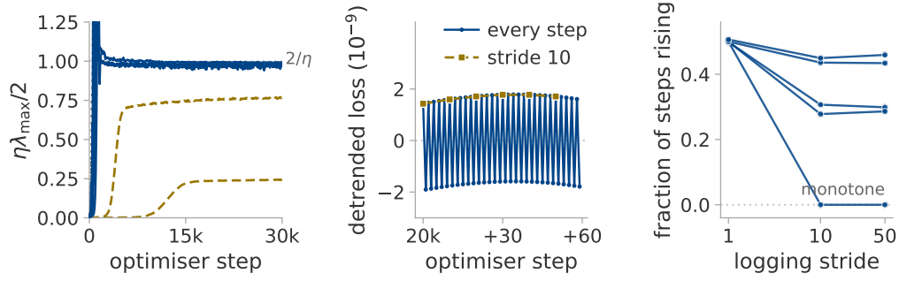
Figure 11: Whether full-batch descent reaches the edge of stability, and what the logging stride removes. (a) The stability ratio along training, seed 1 of each rate; the seeds agree to within the linewidth. Rates below the dotted line descend monotonically and are drawn as transients; those that pin against it are at the edge. (b) Sixty consecutive steps at \eta = 2 \times 10^6 , against the same series at a stride of ten: the two-cycle is not blurred by that stride but removed by it. (c) The fraction of steps on which the loss rises, for each edge-of-stability rate, against the logging stride.
