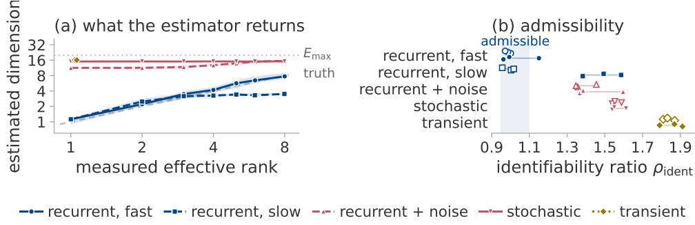
Figure 1: Recovery of the active dimension, and where it fails. Five of the nine excitation cases of section 5.2; colour is the regime of section 3.3. (a) Estimate against truth. Marker, median over four seeds and ten observers; band, their interquartile range; dashed diagonal, exact recovery; dotted line, E_{\max} . (b) The identifiability ratio at two ranks, open marker r = 2 , solid r = 6 , one per observer.
