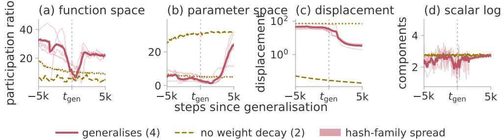
Figure 2: Simplification of the trajectory at generalisation. Three regularised seeds of modular addition and one S_5 composition against the same two configurations without weight decay, aligned on the generalisation step of the run each matches. Thick line, the mean of the four that generalise; band, the two-hash disagreement (Appendix G.1). Panels (a)–(c) plot \text{PR}^{\text{det}} over windows of 600 steps, 300 for S_5 ; (d) is the delay estimate of section 7.3 at the same midpoints.
