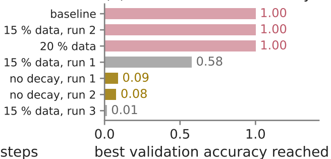
(b) Best validation accuracy
