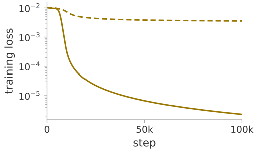
(b) the (2n_1+3n_2)^4 pair
