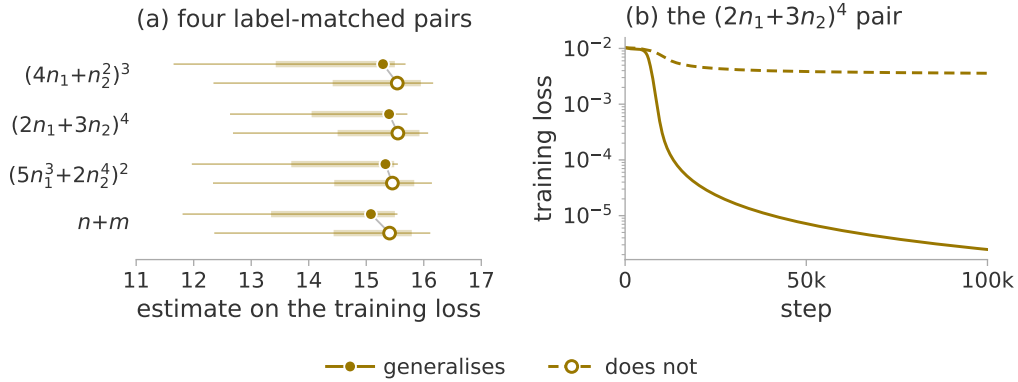
Figure 8: The estimate tells apart two targets that fit the training set alike, only one of them representable by the architecture. (a) The four pairs of section 7.1, on the training loss. Marker, median over the sliding windows; thick bar, interquartile range; thin line, full range. All runs are transient, hence one colour; fill and dash mark generalisation. (b) One pair in full: the representable target drives the loss orders of magnitude lower.
