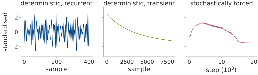
Figure 11: The three regimes as raw scalar logs. Each panel is the parameter norm, standardised to zero mean and unit variance as in Algorithm 1. Left, the constrained head of section 5.2 under fast quasiperiodic forcing, recurrent on a torus. Middle, the same system under plain gradient descent, transient over its whole record. Right, a transformer grokking modular addition, stochastically forced.
