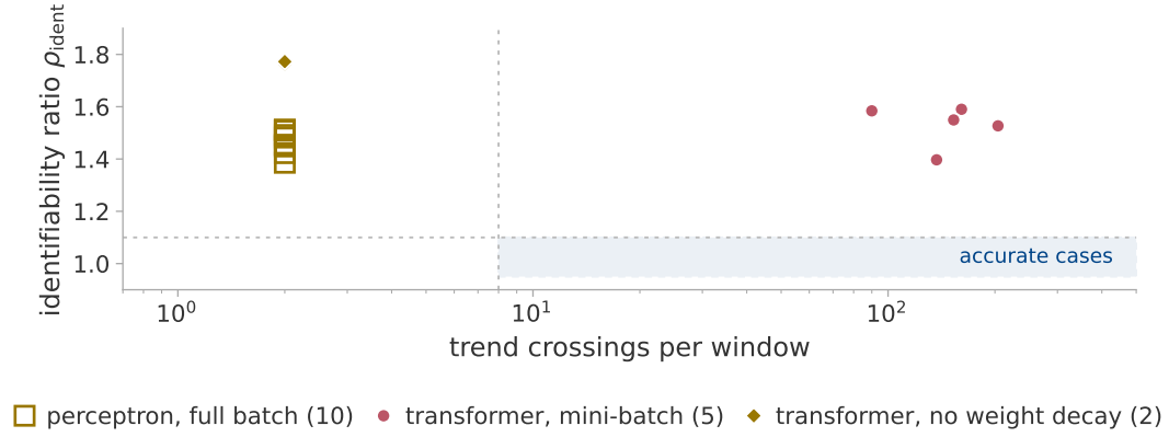
Figure 7: No grokking log lies where the estimate was accurate. Every log of section 7 in the plane of the identifiability ratio and the trend-crossing count, the transformer runs observed through the parameter norm and the perceptron runs through the training loss. Colour is the regime of section 3.3, marker shape the setting. The shaded rectangle is where every accurate case of section 6 fell. It is a record of those cases, not a test.
