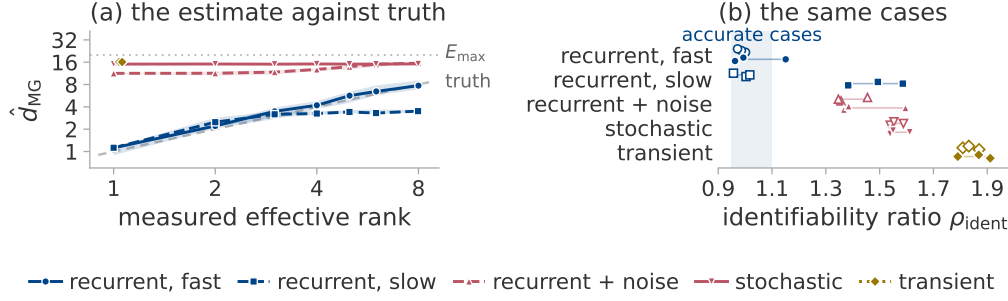
Figure 1: Recovery of the active dimension in each regime. The linear head of section 5.2 under five excitations: two quasiperiodic forcings at different rates, the fast one with gradient noise added, mini-batch noise alone, and plain gradient descent. Colour is the regime of section 3.3. (a) Estimate against truth: marker, median over seeds and observers; band, their interquartile range; dashed diagonal, exact recovery; dotted line, E_{\max} . (b) The identifiability ratio on the same five cases, one point per observer, at r = 2 (open) and r = 6 (solid).
