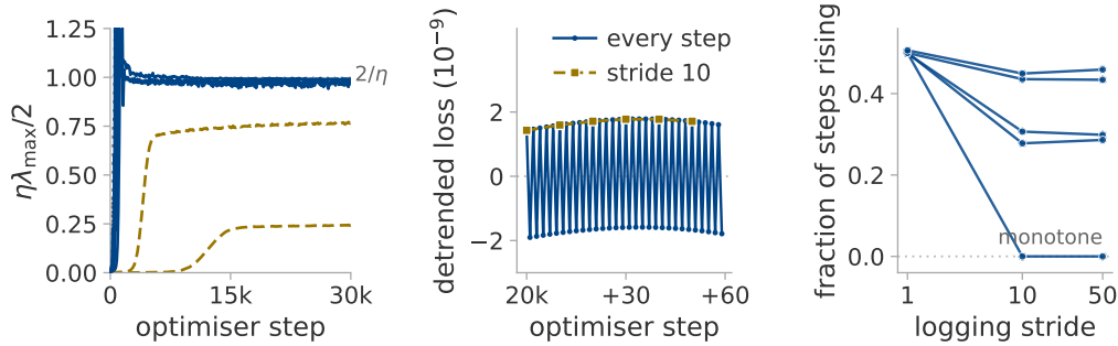
Figure 13: Full-batch descent reaches the edge of stability. (a) The stability ratio along training, one seed per rate. (b) Sixty consecutive steps at one rate at the edge, against the same series at a stride of ten: the two-cycle is removed by that stride rather than blurred by it. (c) The fraction of steps on which the loss rises, against the logging stride.
