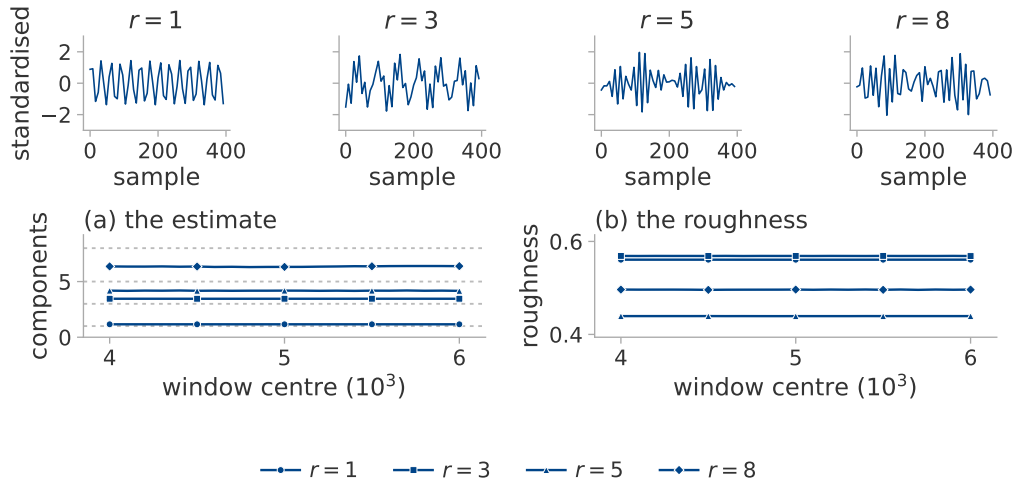
Figure 4: Four logs that look alike, separated by the estimator. The image-data system of section 5.2 at four ranks and a seed the configuration was not selected on, through the parameter norm. Above, four hundred samples of each log. (a) The estimate over sliding windows, the measured effective rank dotted. (b) The roughness of the same windows.
