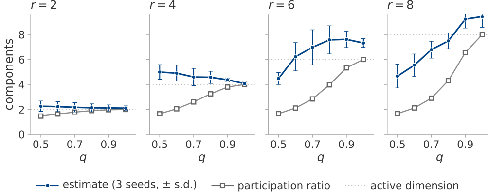
Figure 6: The estimate follows the active dimension, not the effective rank. Forcing phase l at amplitude q^l holds the active dimension at r while the effective rank falls with q . The system of section 5.1, three seeds, one panel per r ; the dotted line is r . Filled circles, the estimate, median over seeds, with standard deviation as bars; open squares, the measured effective rank, which matches its closed form to two decimals and so has no spread.
