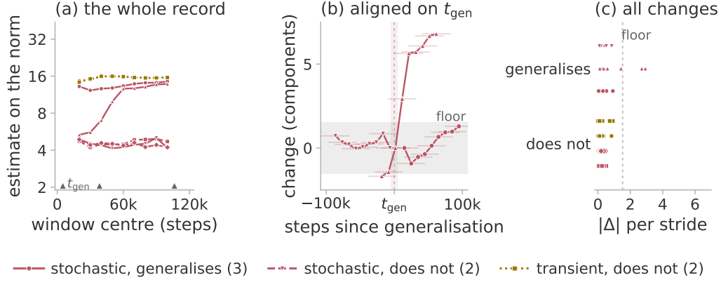
Figure 10: The frozen window localises a feature only to \pm 20\,000 steps. The estimate on the parameter norm for the seven extended runs, under the frozen configuration of section 7.1, plotted at the window centres. Colour is the regime of section 3.3. (a) Every window, with the generalisation steps marked on the axis. (b) The generalising runs aligned on their own generalisation step. (c) All the changes from one stride to the next, one sub-row per run. The grey band in (b) and (c) is the floor a ramped gain alone produces (section 6.3).
