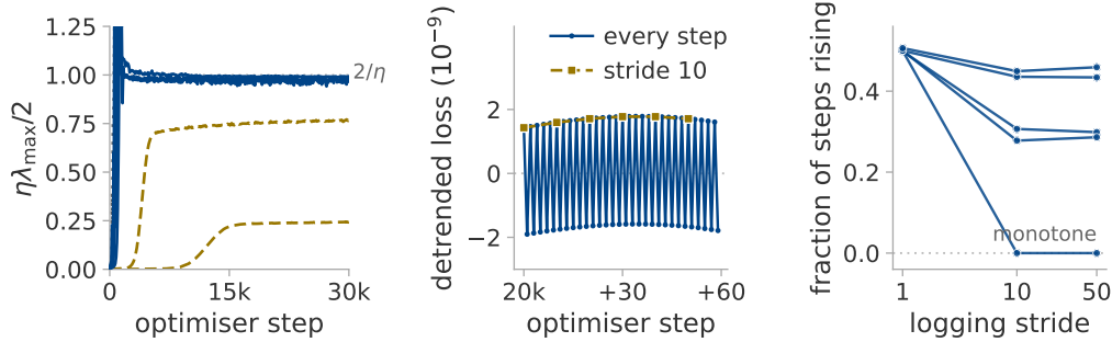
Figure 13: Full-batch descent reaches the edge of stability. (a) The stability ratio along training, one seed per rate. (b) Sixty consecutive steps at one rate at the edge, against the same series at a stride of ten: the two-cycle is removed by that stride rather than blurred by it. (c) The fraction of steps on which the loss rises, against the logging stride.
