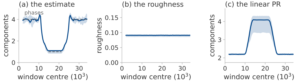
Figure 14: A change in the number of independent phases, tracked as it happens. The harmonic control of this appendix, scheduled from four phases to one and back; median over eight seeds, band and their range. Dashed in (a), the number of phases, drawn only where no ramp reaches into the window. Panel (b) is the roughness, which the construction holds fixed; the linear statistic of (c) moves in the opposite direction.
