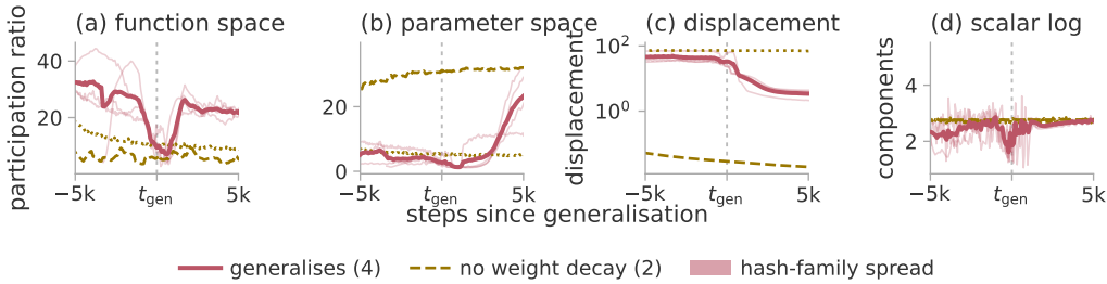
Figure 2: Simplification of the trajectory at generalisation. Three regularised seeds of modular addition and one S_5 composition, against the same two configurations without weight decay, each aligned on the generalisation step of the run it matches; colour is the regime of table 1, the thick line the mean of the four that generalise. The statistic in (a)–(c) is \text{PR}^{\text{det}} , an effective rank: none of these runs recurs, so none supports a dimension. Windows are 600 optimiser steps, 300 for S_5 , and the band on (a) and (b) is the two-hash disagreement (Appendix I). Panel (d) is a different measurement at the same midpoints, the delay estimate of section 7.3 on the parameter-norm log.
