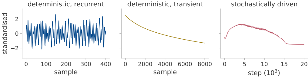
Figure 10: What the estimator is given in each regime. The three regimes of table 1 as raw scalar logs, standardised as the estimator standardises them. Left, the recurrent case of this appendix, whose orbit closes onto a torus. Middle, the transient case over its whole record, a decay that increases on none of its eight thousand steps. Right, a mini-batch transformer run through the parameter norm. The last two are the ones the diagnostics of section 3.4 must reject, and the difference between them is why one statistic will not do it: the transient is monotone and the driven run is not, so a test of non-monotonicity catches the first and a test of embedding stability the second.
