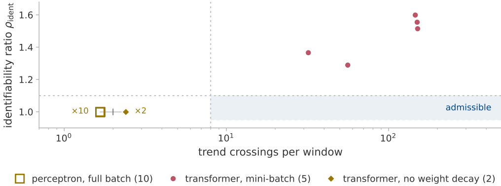
Figure 6: Whether any training log of either setting is admissible. Every log of section 7 in the plane of the two diagnostics, one point per run: seven transformer runs observed through the parameter norm, ten perceptron runs through the training loss. Colour is the regime of table 1 and marker shape the setting. The vertical axis is the identifiability ratio, near unity when the estimate does not depend on the embedding dimension; the horizontal axis is the trend-crossing count. Twelve runs coincide at two crossings with \rho_{\text{ident}} near unity; those groups are drawn with a small offset either side of the true abscissa, which the grey tick marks, and labelled with their multiplicity. The shaded rectangle is where every accurate case of section 6 fell. It describes the calibration and is not a decision rule.
