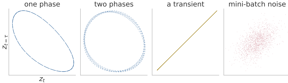
Figure 4: The set the neighbour search measures, in the plane of the first two delay coordinates. One window of the image-data system of section 5.1 under each excitation, reconstructed at the frozen configuration. A single phase closes an orbit, two fill a surface, a converging run never returns, and mini-batch noise fills the space it is given.
