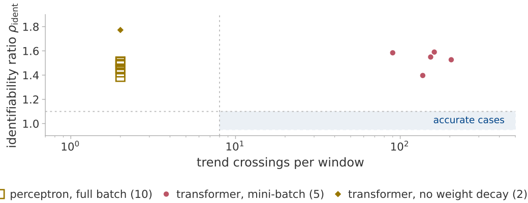
Figure 8: No grokking log lies where the estimate was accurate. Every log of section 7 in the plane of the identifiability ratio and the trend-crossing count, the transformer runs observed through the parameter norm and the perceptron runs through the training loss. Colour is the regime of section 3.4, marker shape the setting. The shaded rectangle is where every accurate case of section 6 fell. It is a record of those cases, not a test.
