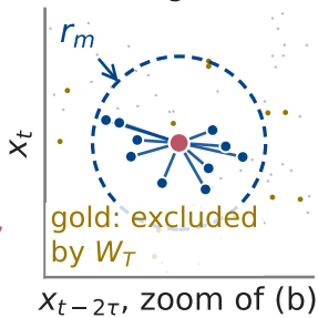
(c) Neighbours
