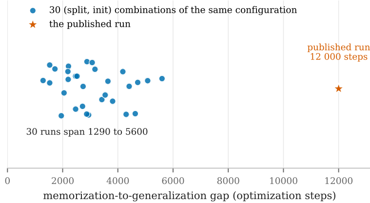
Figure 9: Memorisation-to-generalisation gap for thirty runs of one configuration, varying only the split and initialisation seeds. Every run generalises and every gap lies between 1290 and 5600 steps. The delay reported in earlier work lies far outside this distribution.
