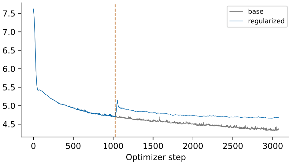
MG input: fixed-probe reconstruction NLL/token
