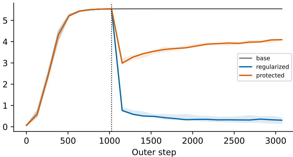
Observed reconstruction NLL/token
