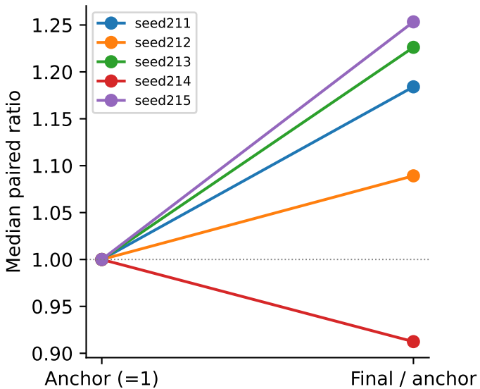
Full-state recurrence error R
