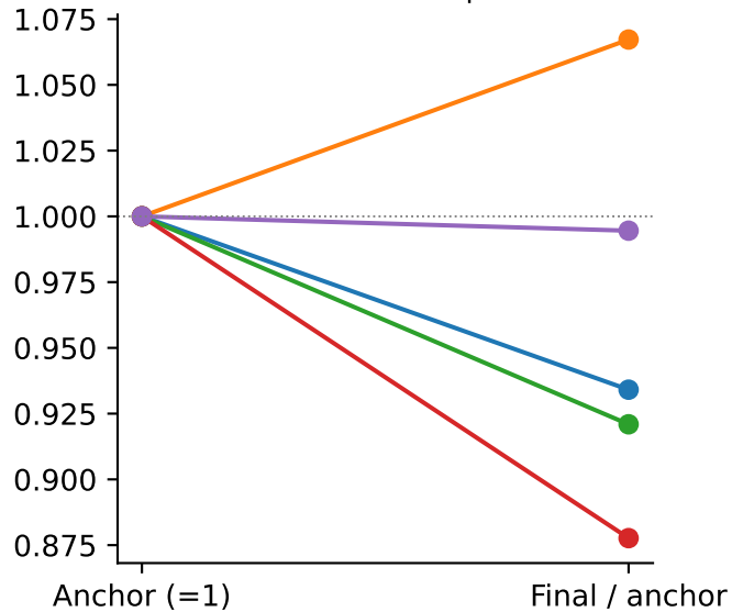
Full-state section dispersion D
