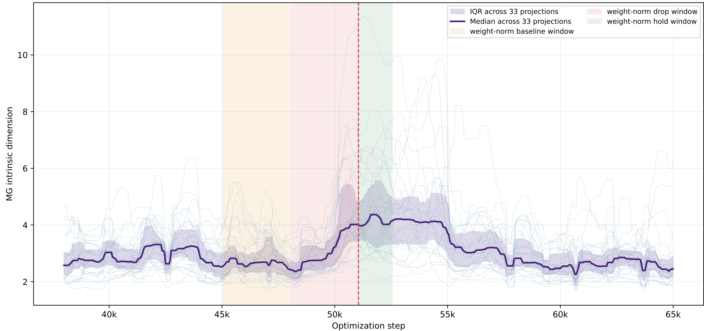
Weight-projection MG dimensions around the weight-norm trigger
