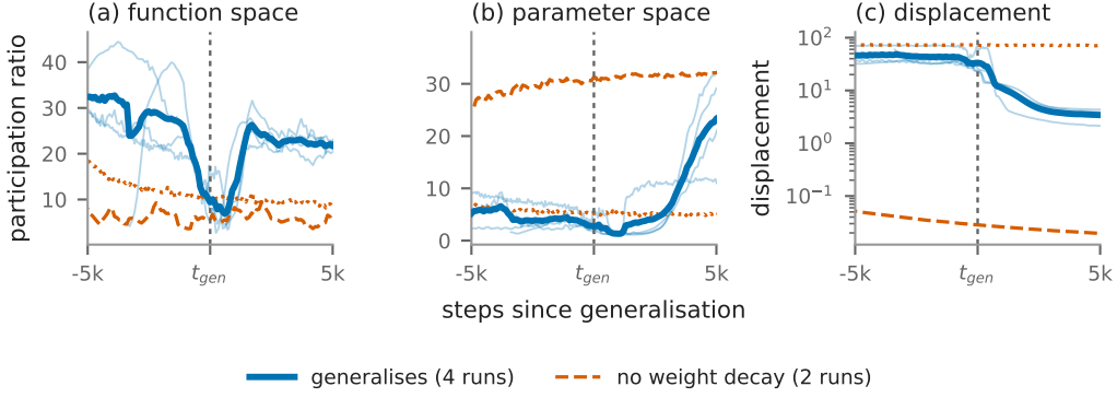
Figure 3: The trajectory effective rank measured directly (section 7.3), on six transformer runs: three seeds of modular addition at weight decay 1.0 and one S_5 composition at 0.2, against the same two configurations at weight decay zero, which memorise and stay at chance validation accuracy for their whole budget. The statistic is PR^{\det} of section 3.1, an effective rank; these runs have no recurrent set, so no active dimension is defined for them. Windows of 600 steps at their midpoint, so the window is not causal and a feature is located to within \pm 300 steps; each control, having no generalisation step, is aligned on that of the matched weight-decay run (Appendix G). Thick blue is the mean of the four generalising runs, thin blue the runs themselves.
